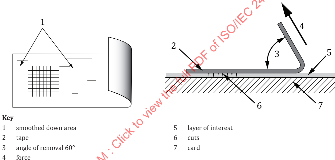
Figure 12 — Positioning the adhesive tape
