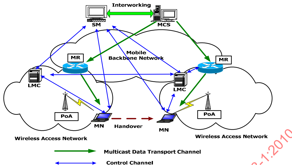
Figure 5 – Reference configuration of MMC functional entities in multicast networks
