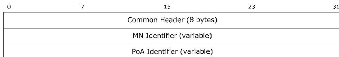
Figure 26 – Handover initiation request
