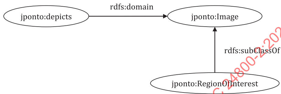
Figure 3 — The jponto:depicts property allows binding an image with the real-world objects and events that it represents
