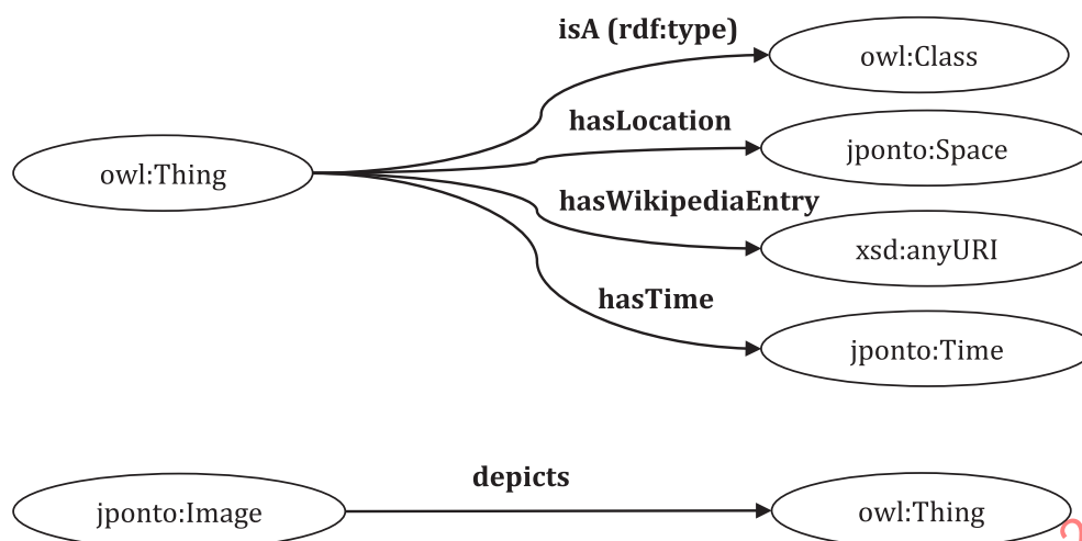
Figure 8 — Generic properties of JPonto-visual (arrows show the domain and range of the property)
