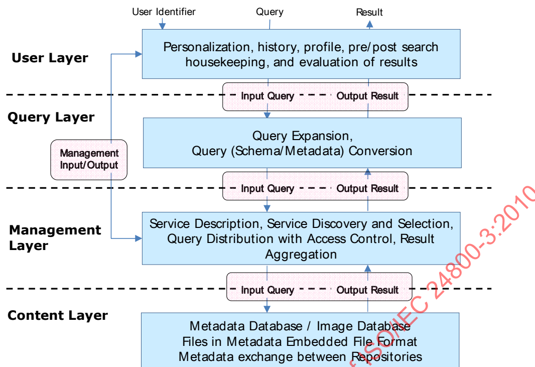
Figure 1 — JPSearch architecture and scope of this part of ISO/IEC 24800
