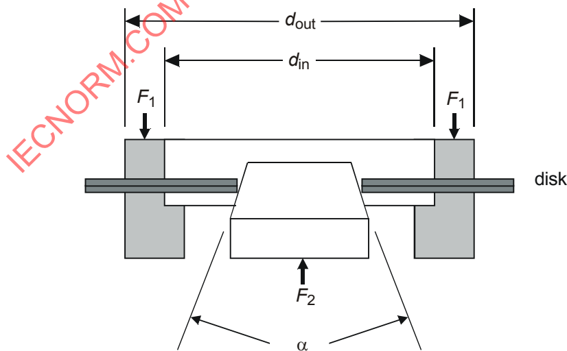
Figure 3 — Clamping and chucking conditions
