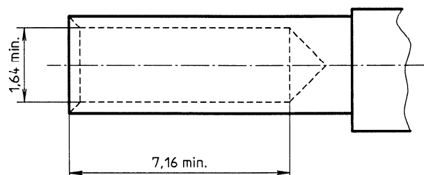
Figure 5 — Female contact
