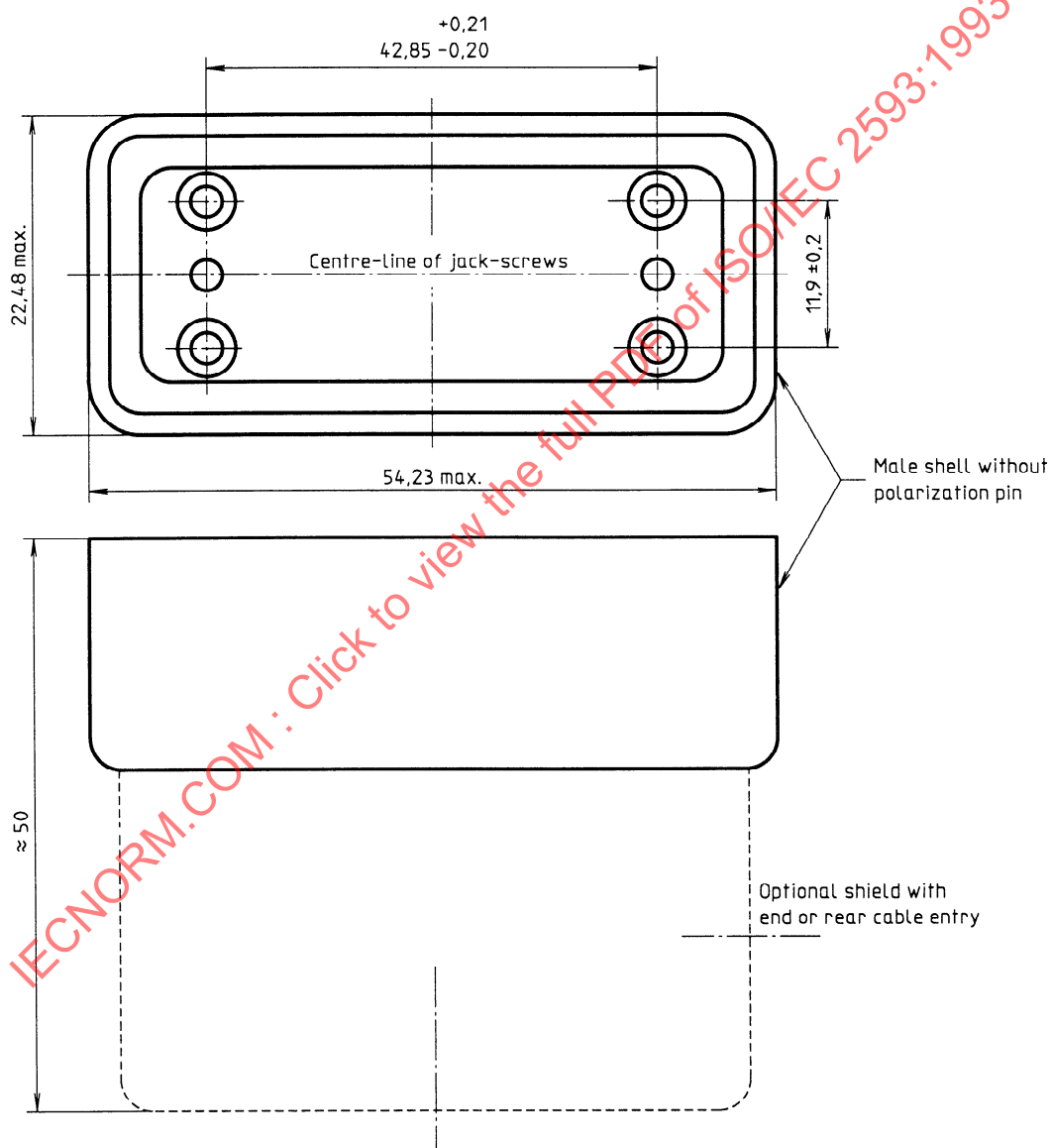
Figure 1 — DTE connector
