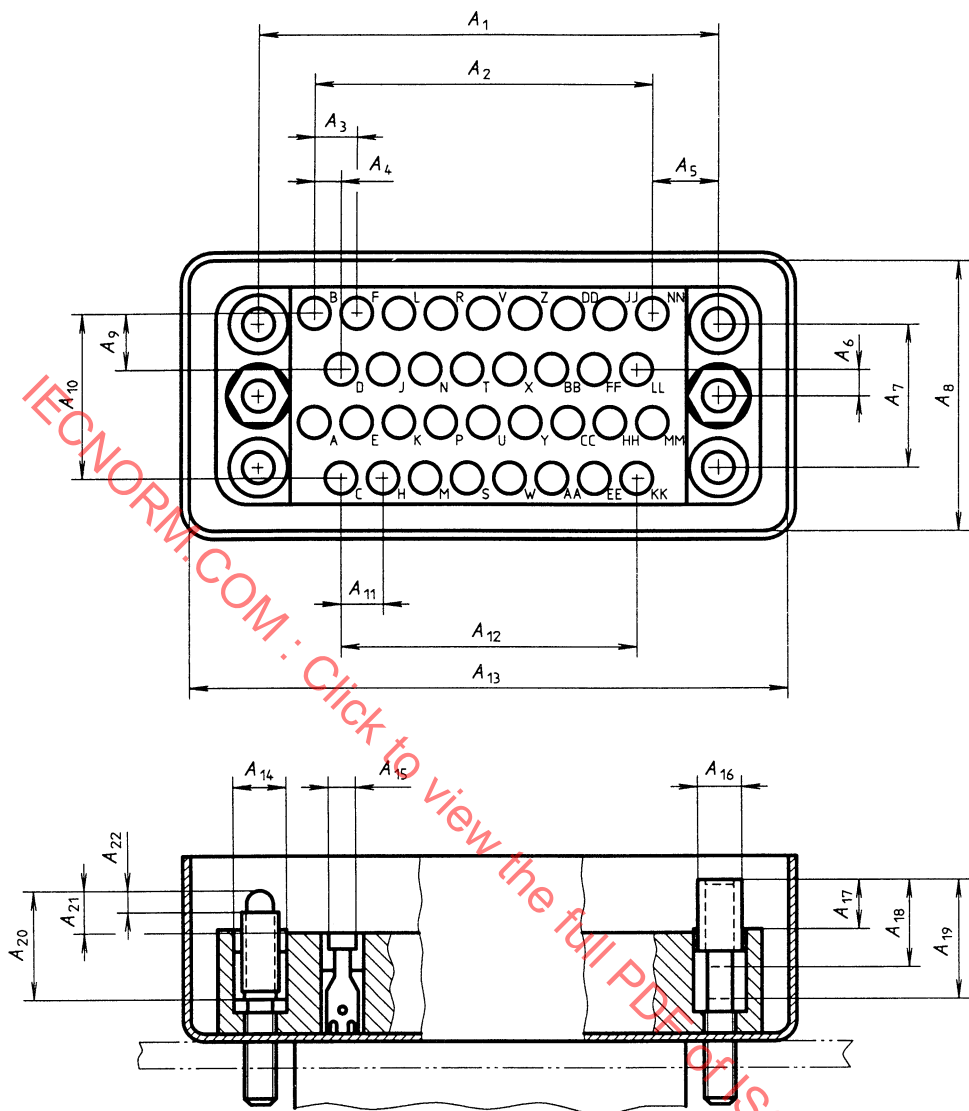
Figure 6 — DTE connector
