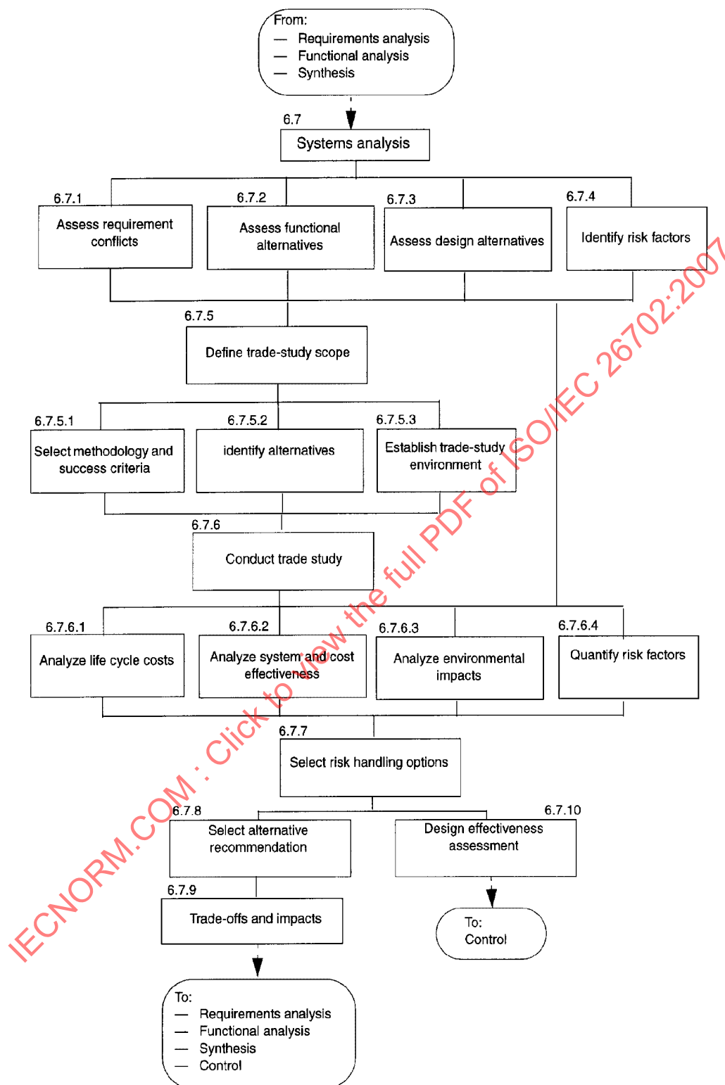
Figure 16—Systems analysis process
