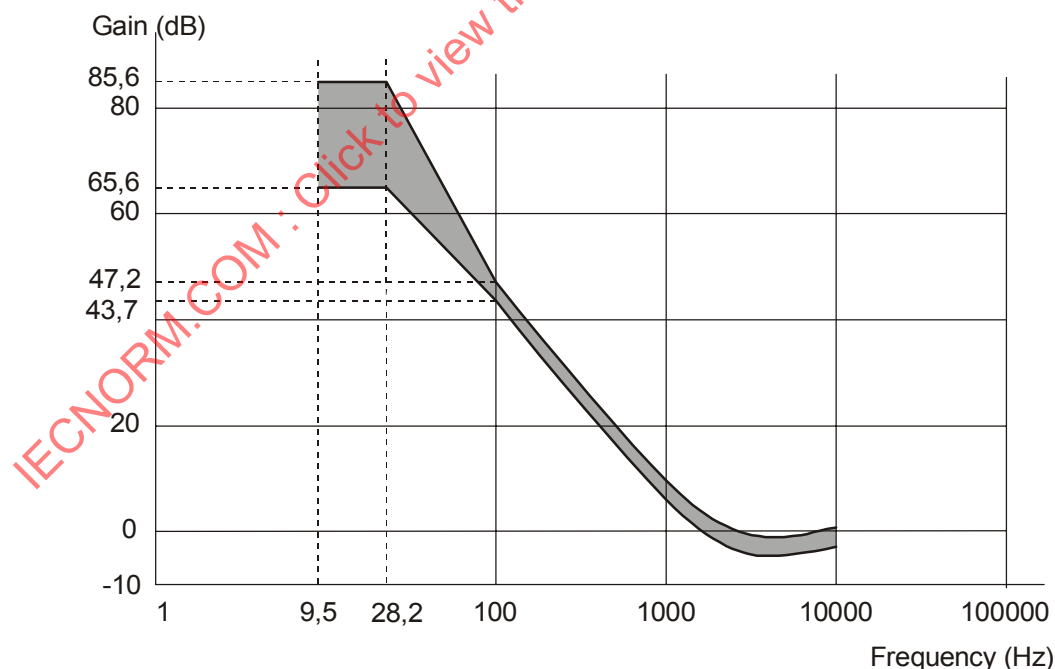
Figure 5 — Reference servo for radial tracking
