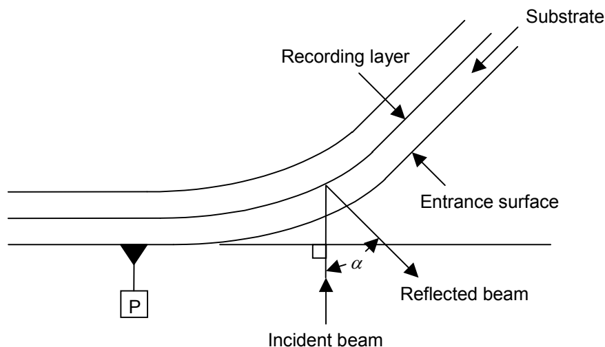
Figure 9 — Angular deviation
