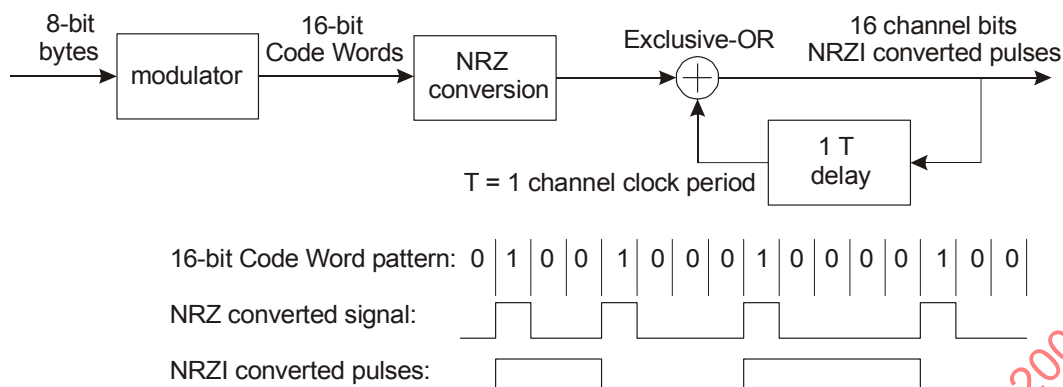
Figure 15 — NRZI conversion
