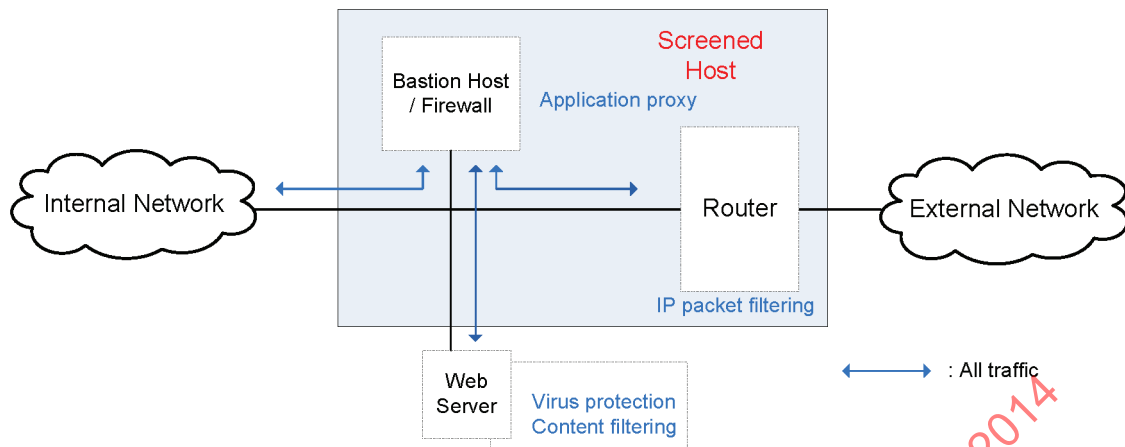
Figure 5 — Screened host
