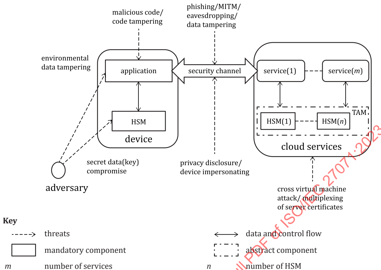
Figure A.1 — Threats on trusted connection
