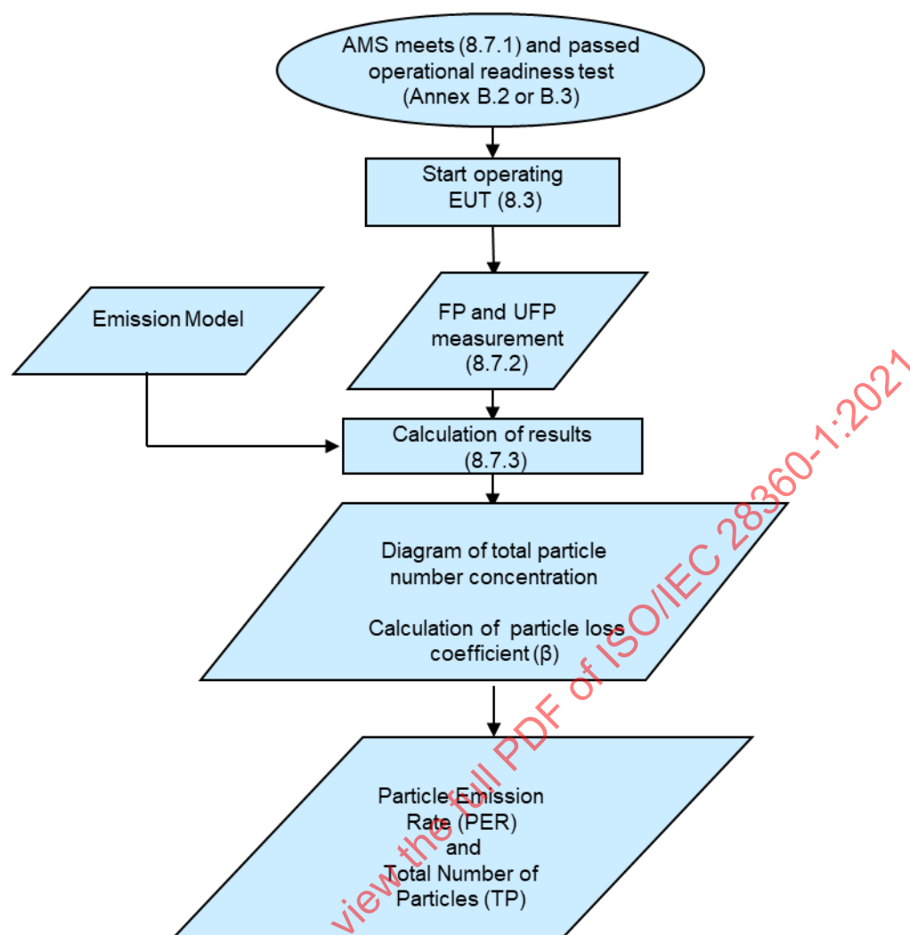
Figure 5 — Determination method for FP and UFP emissions
