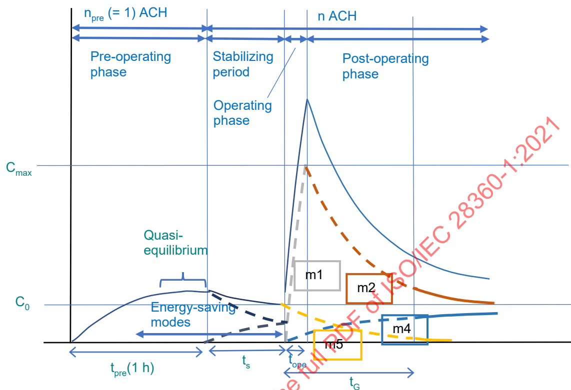
Figure C.1 — Model for QEM
