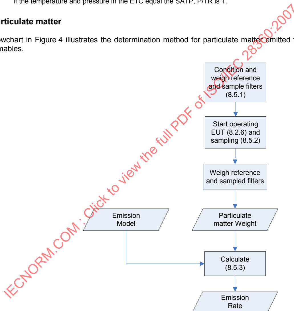
Figure 4 — Determination method for particulate matter
