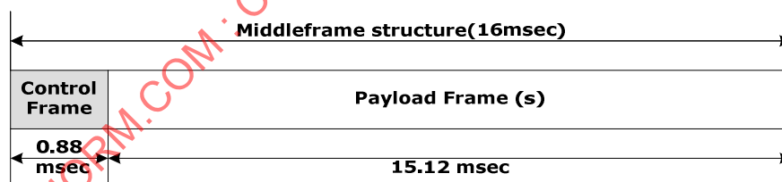
Figure 14 — Middleframe structure
