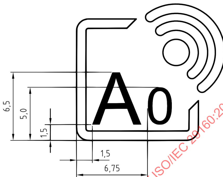
Figure B.4 — RFID Emblem with two-character code
