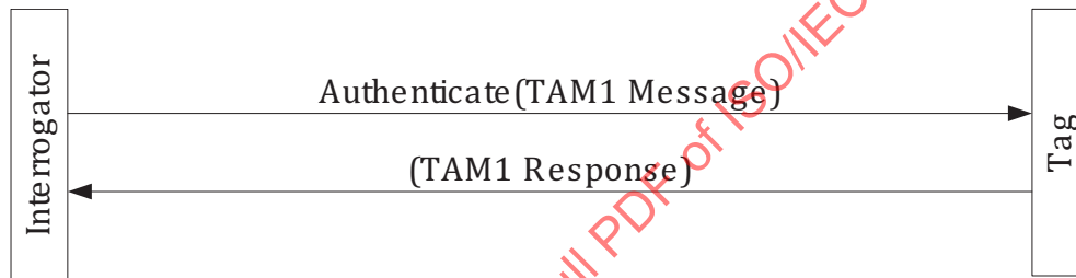
Figure E.1 — Message exchange for Tag authentication
