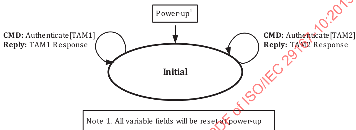
Figure 1 — Crypto suite Tag state diagram
