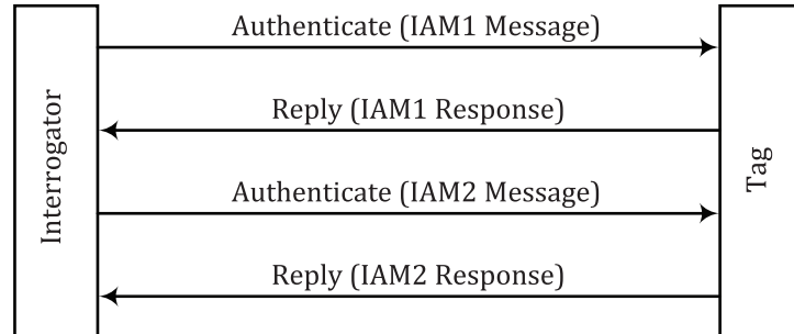
Figure 3 — Interrogator authentication via a challenge-response scheme
