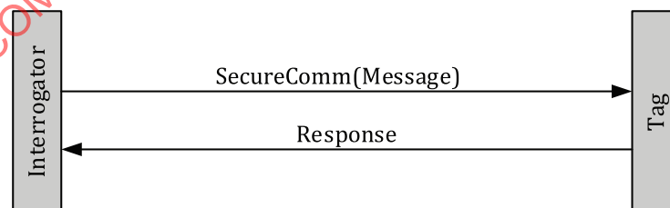
Figure 6 — Secure communication
