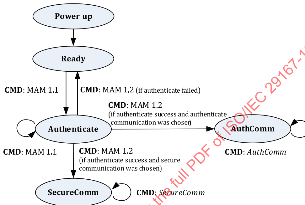
Figure 2 — State diagram
