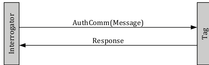
Figure 5 — Authenticate communication
