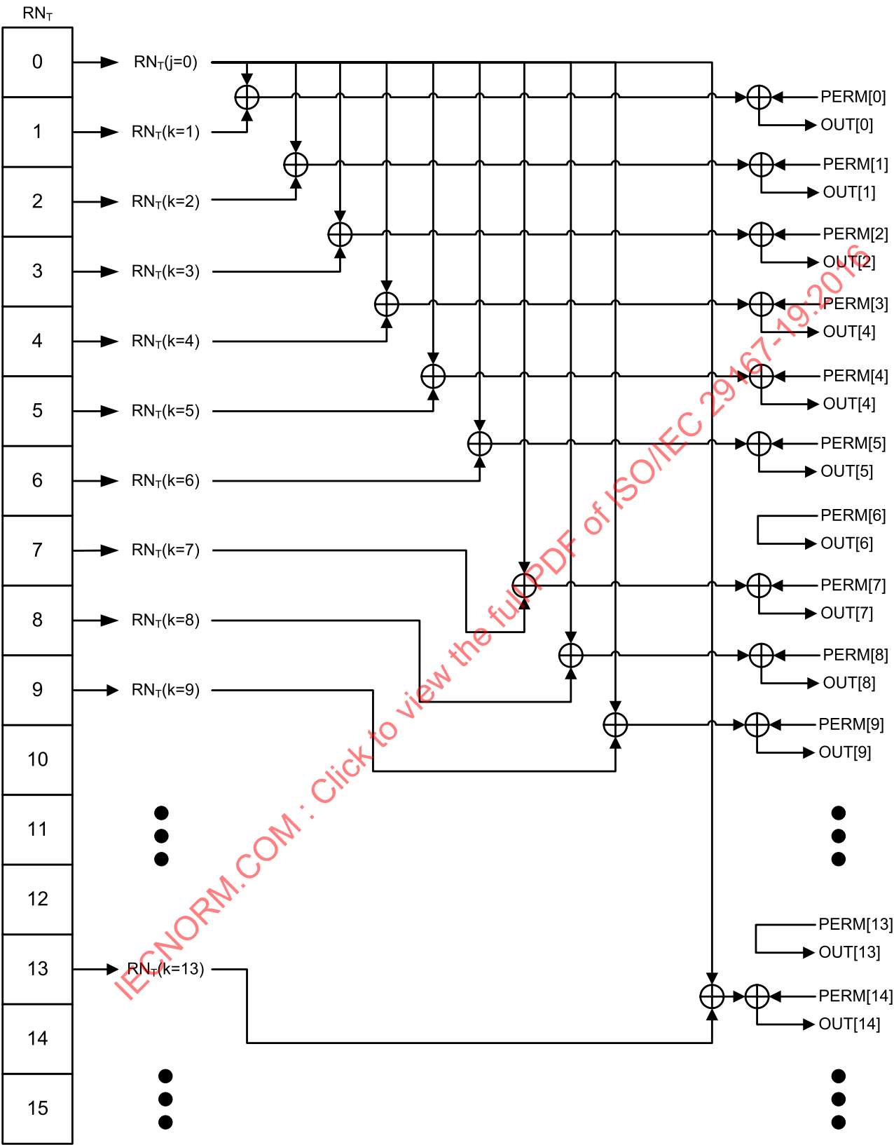
Figure C.2 — Illustration of the application of the mask function
