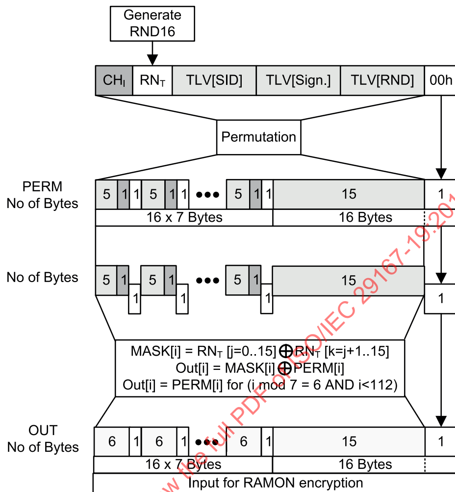
Figure C.1 — Illustration of the mix function
