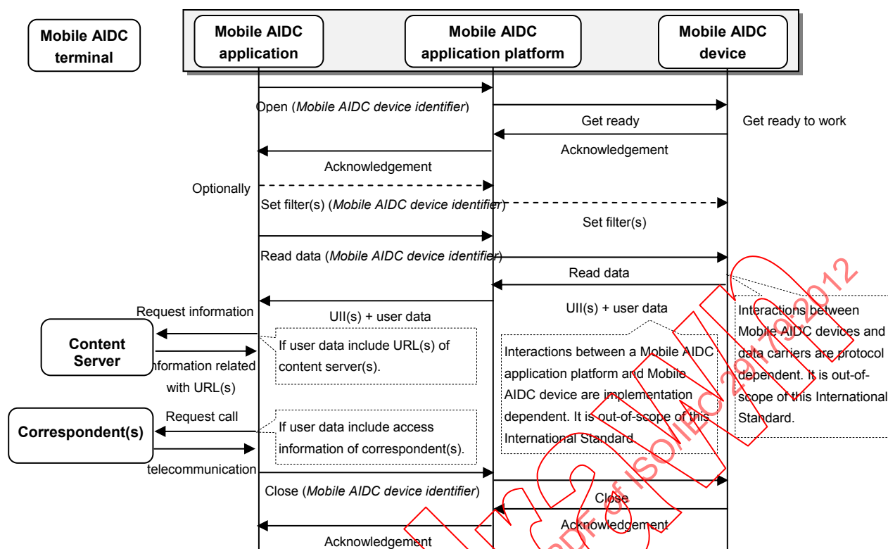
Figure B.2 — Mobile AIDC service scenario: Obtaining relevant information without Ull resolution
