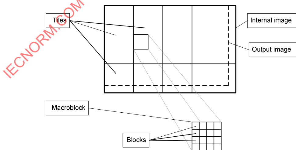
Figure 1 – Informative overview of Image partitions and internal windowing
