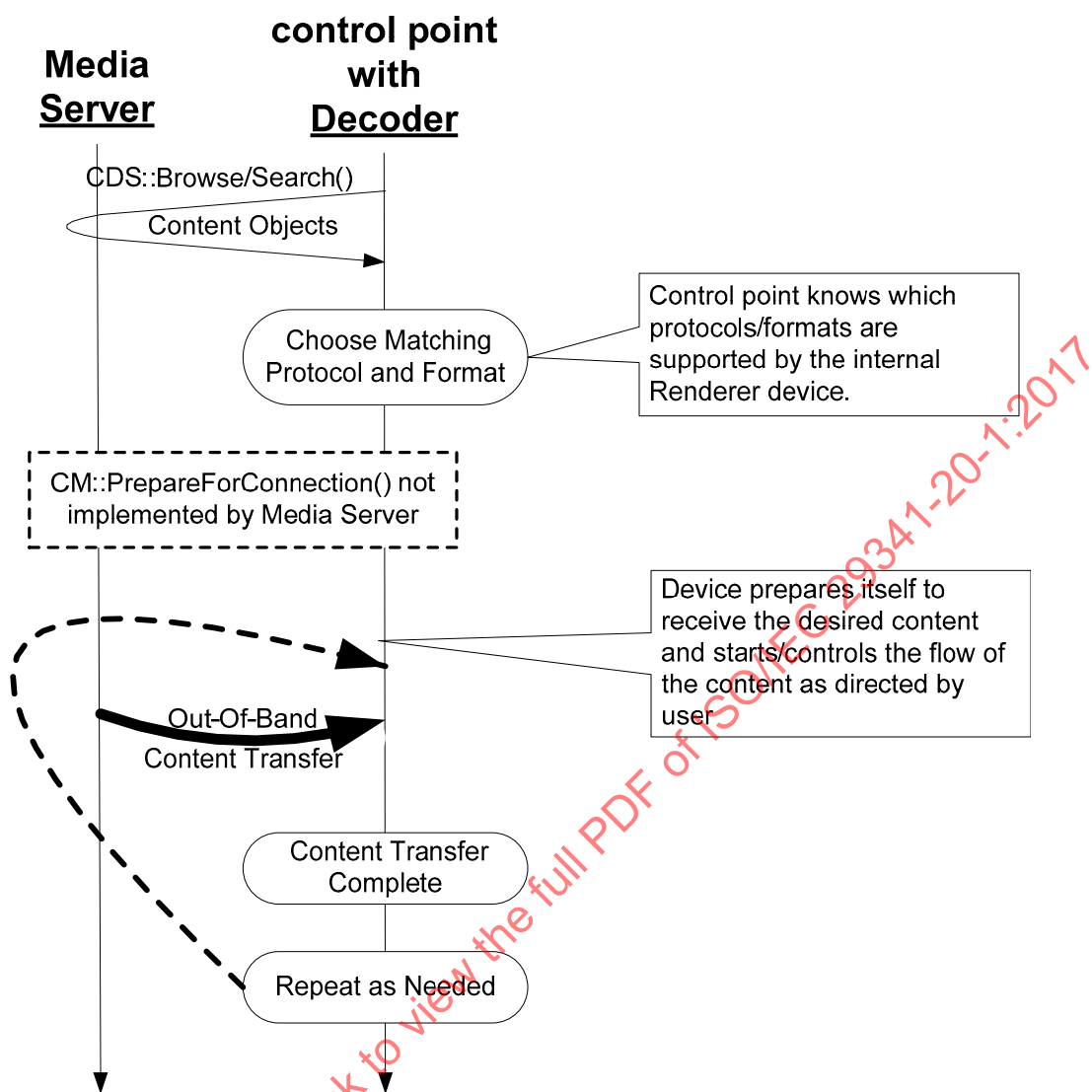
Figure 11 — 2-Box model: Minimal Implementation
