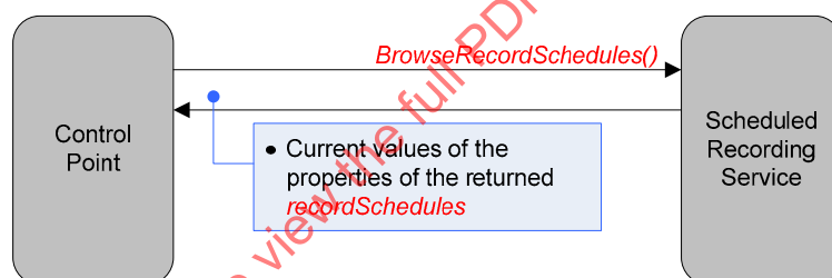
Figure 3 — Browse recordSchedule .
