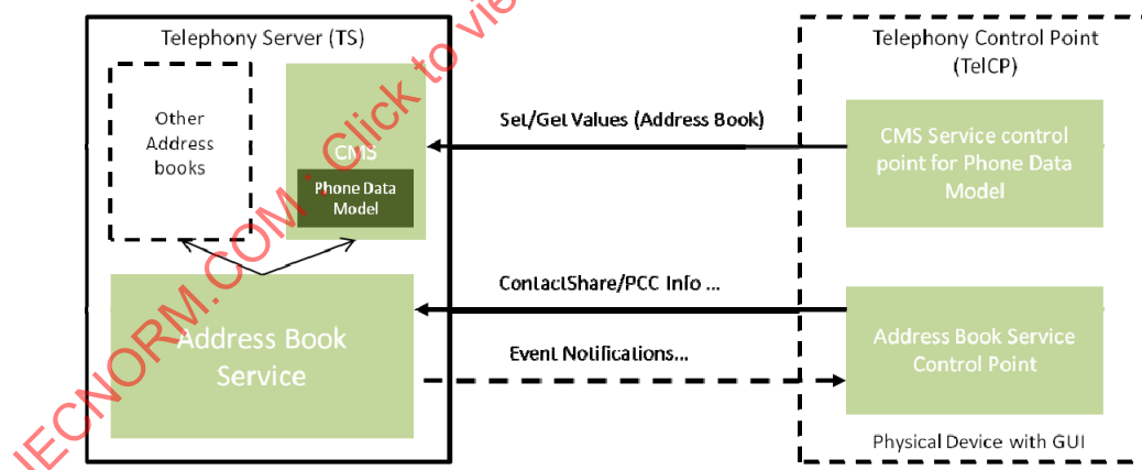
Figure 12 — Architecture for Address Book Service
