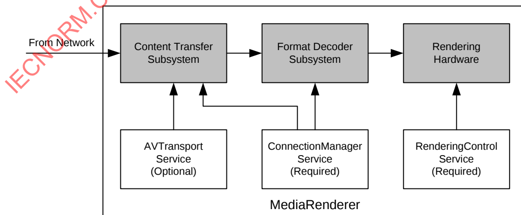
Figure 1 — MediaRenderer Functional Diagram
