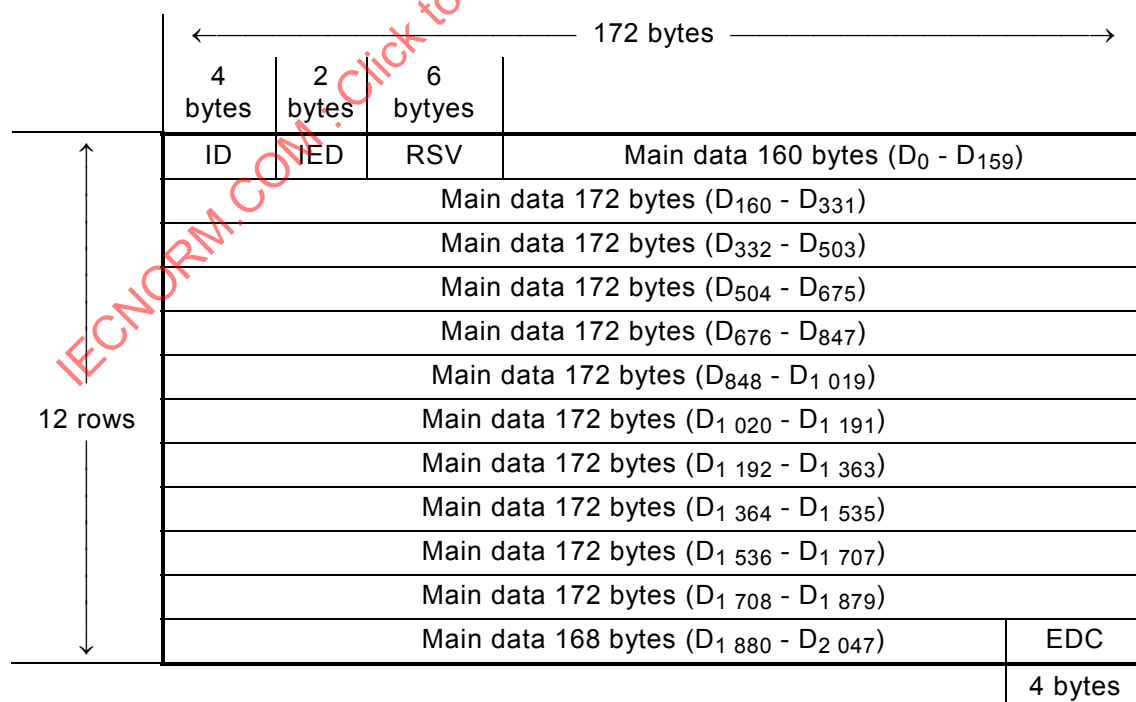
Figure 11 — Data Frame
