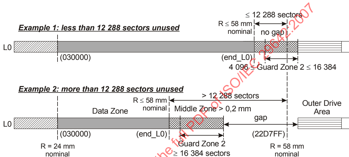
Figure 30 — Two examples of size of Guard Zone 2 on Layer 0 (layout on Layer 1 shall be similar)
