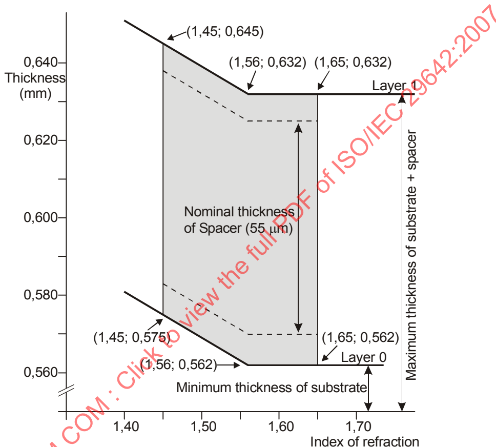
Figure 9 — Thickness of the substrate
