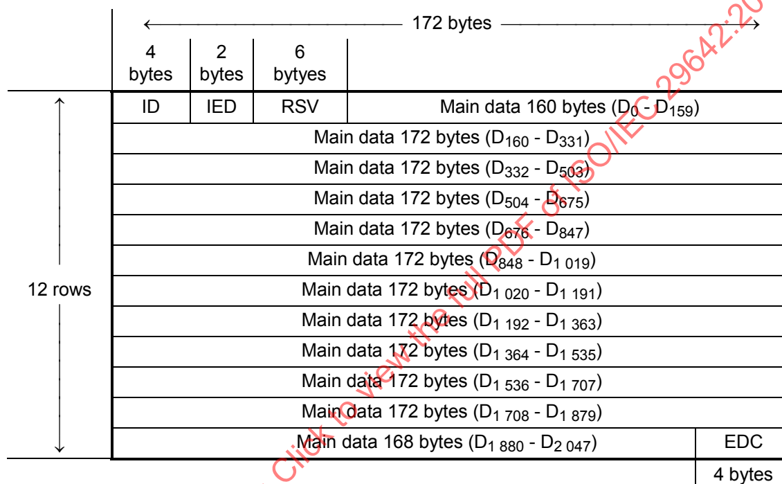
Figure 11 — Data Frame
