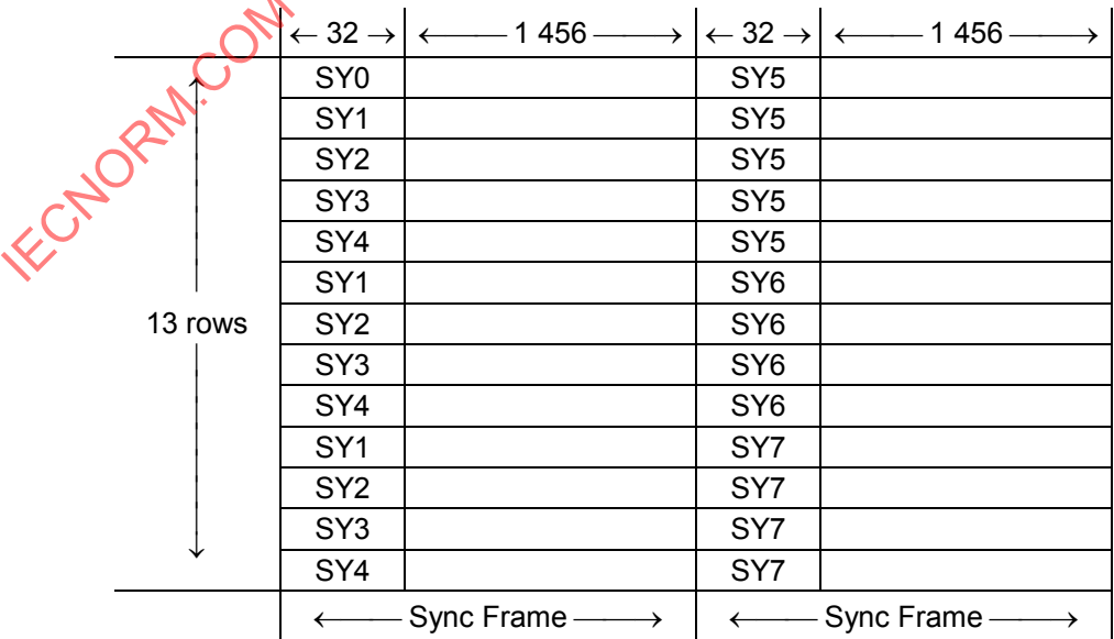
Figure 17 — Physical Sector
