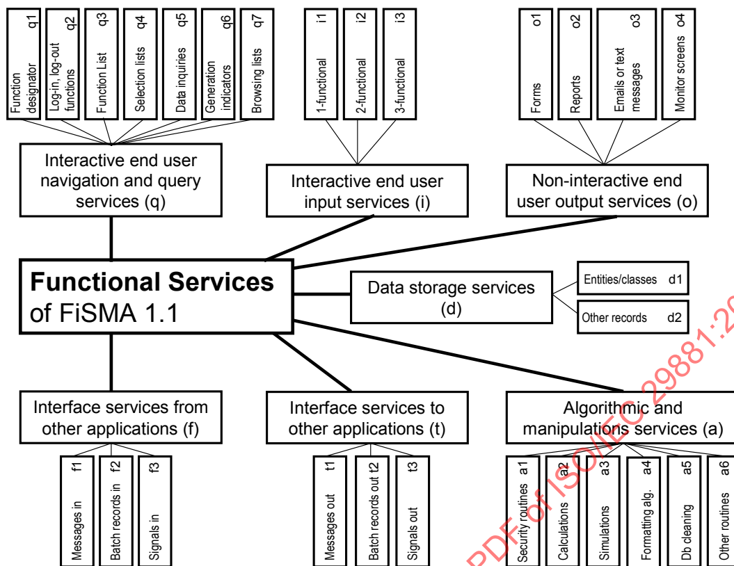
Figure 3 — FiSMA 1.1 BFC classes and BFC types
