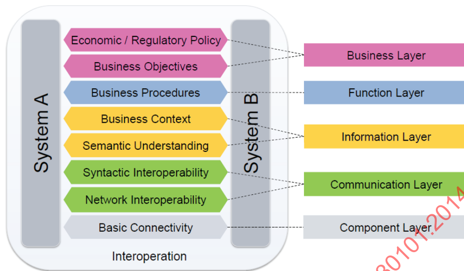
Figure A.6 — Grouping into interoperability layers.
