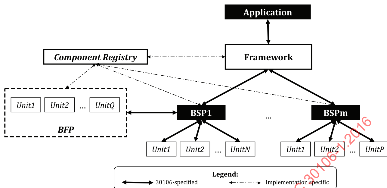
Figure 1 — Generic structure of a framework-based application
