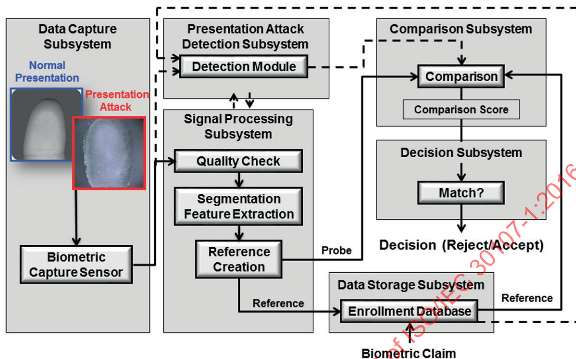
Figure 3 — A general biometric framework with presentation attack detection (other configurations are possible)
