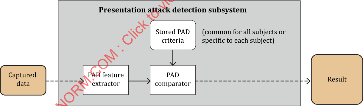
Figure 4 — Components in a general presentation attack detection subsystem
