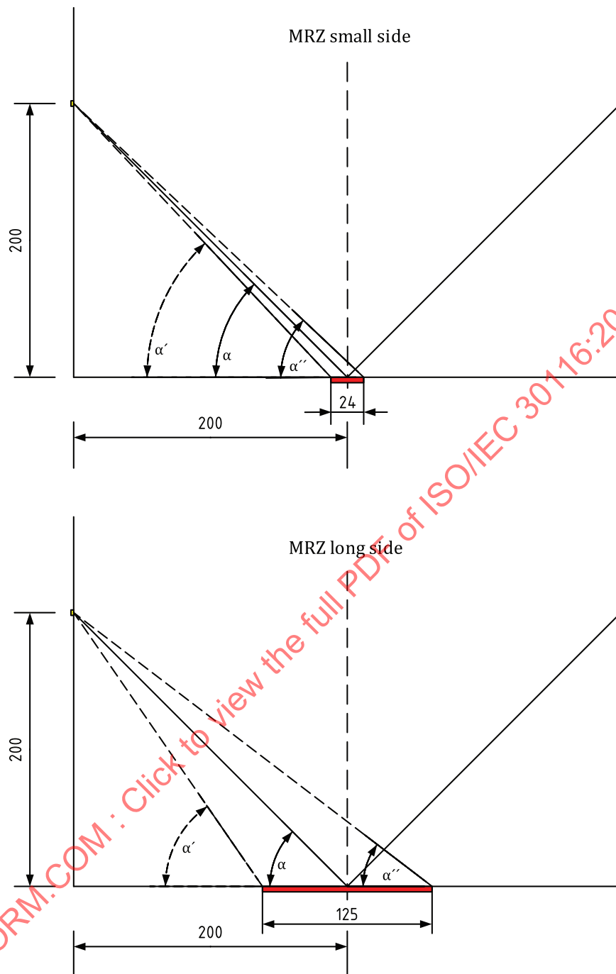
Figure 3 — Reference optical arrangement — Angles and tolerances
