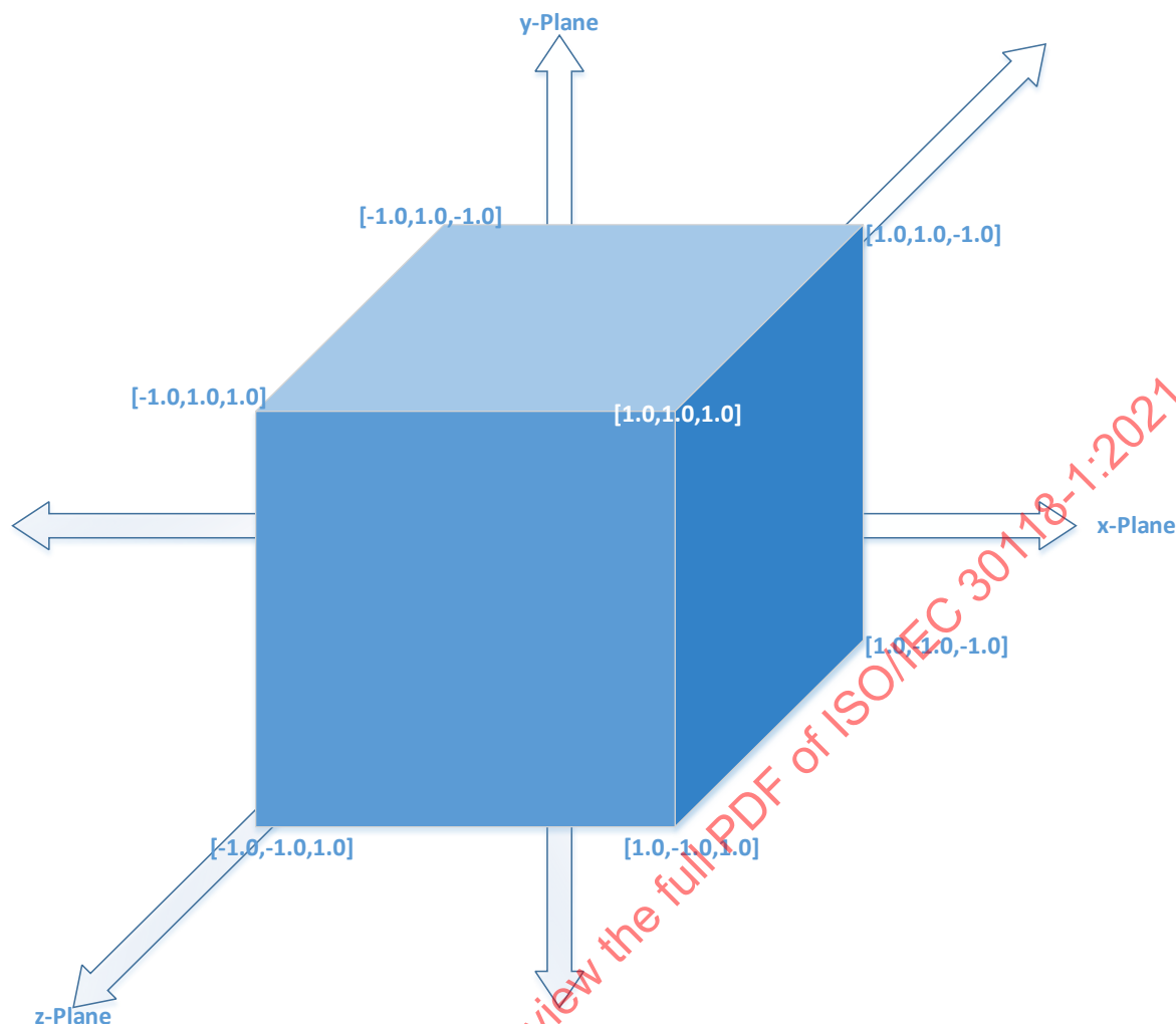
Figure 14 – "tag-pos-rel" definition
