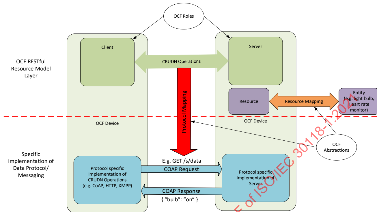
Figure 1 – Architecture - concepts
