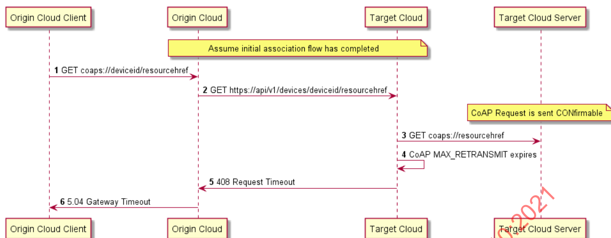
Figure A.6 – Retrieve Resource (timeout) example flow
