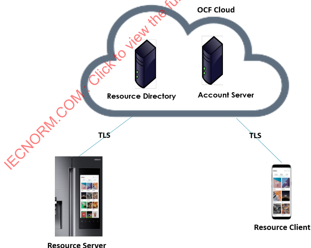
Figure 1 – OCF Cloud Architecture
