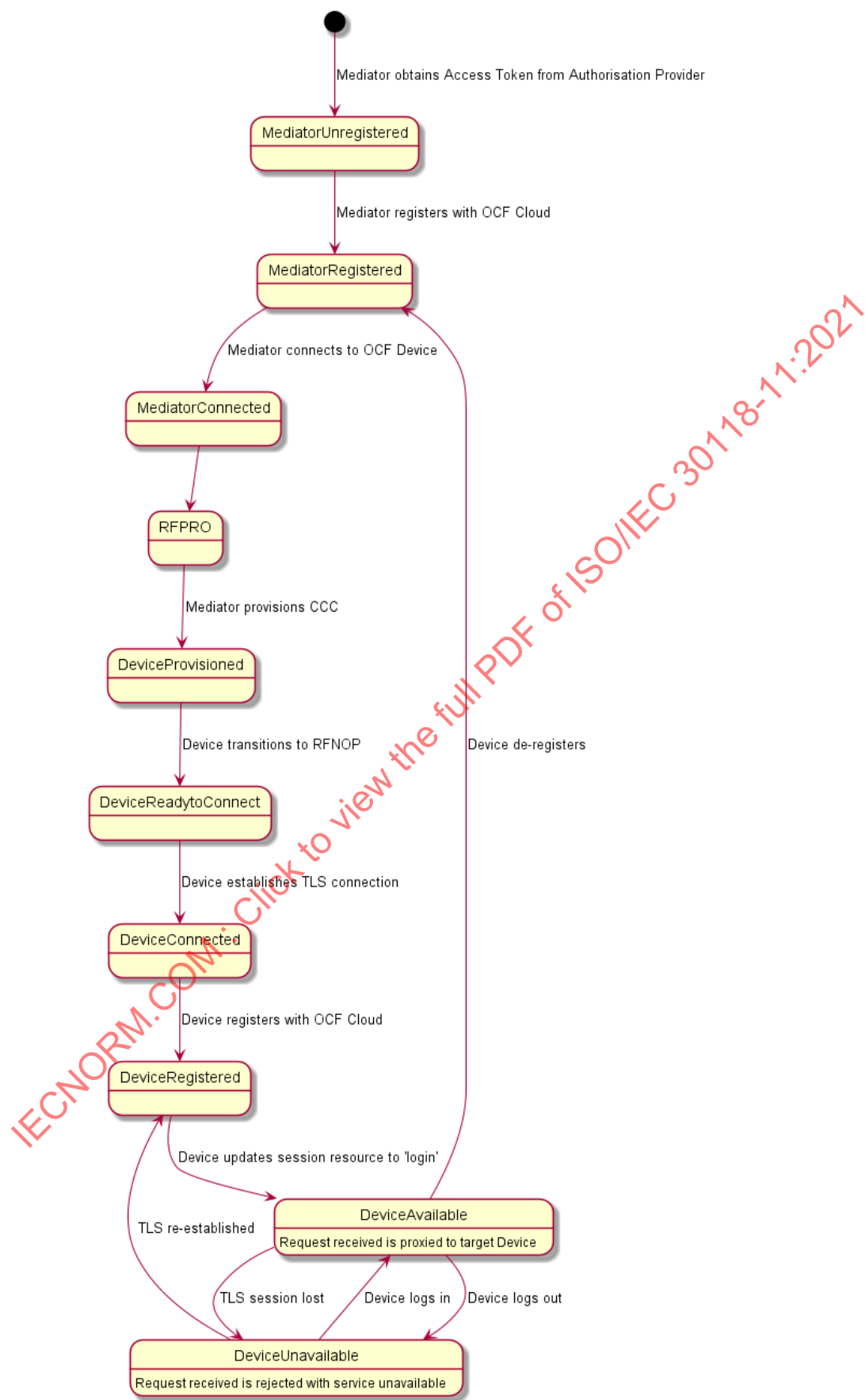
Figure 3 – Overall operational state machine
