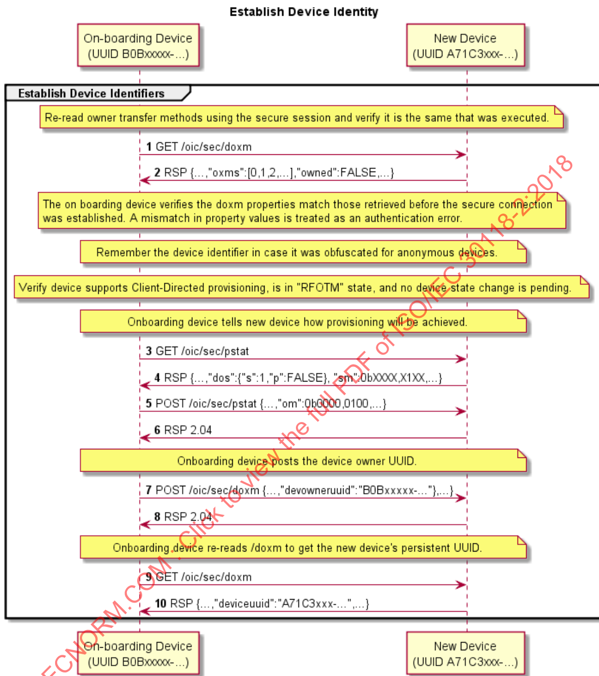
Figure 19 - Establish Device Identity Flow
