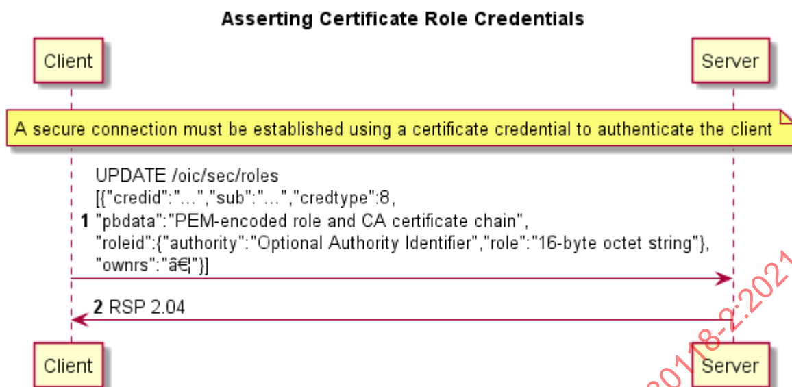
Figure 18 – Asserting a role with a certificate role credential
