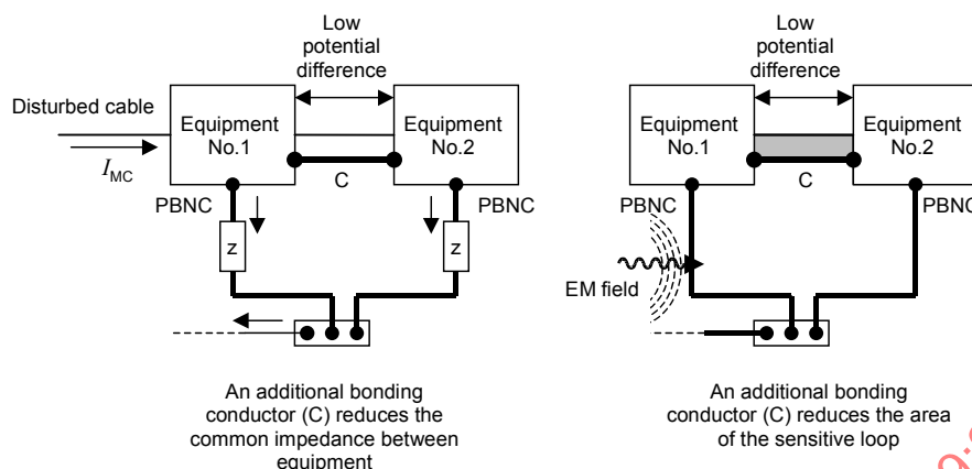
Figure 12 – Example of low common impedance and small loop
