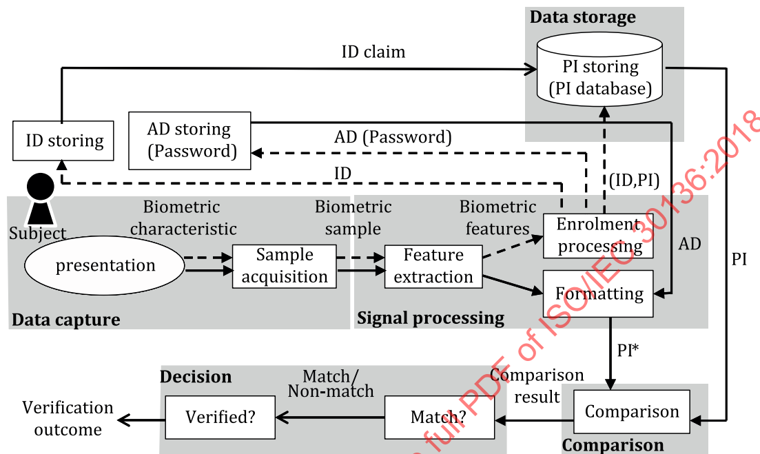
Figure 6 — Application model of password two-factor biometric template protection system
