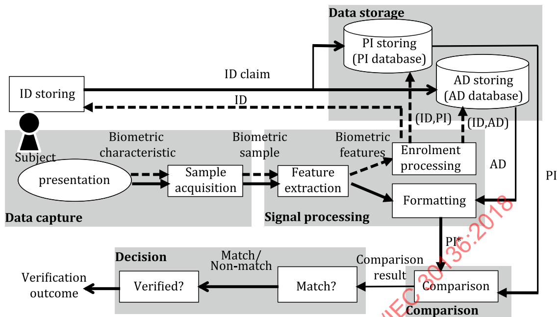
Figure 4 — Application model of biometric template protection system with separate AD and PI databases
