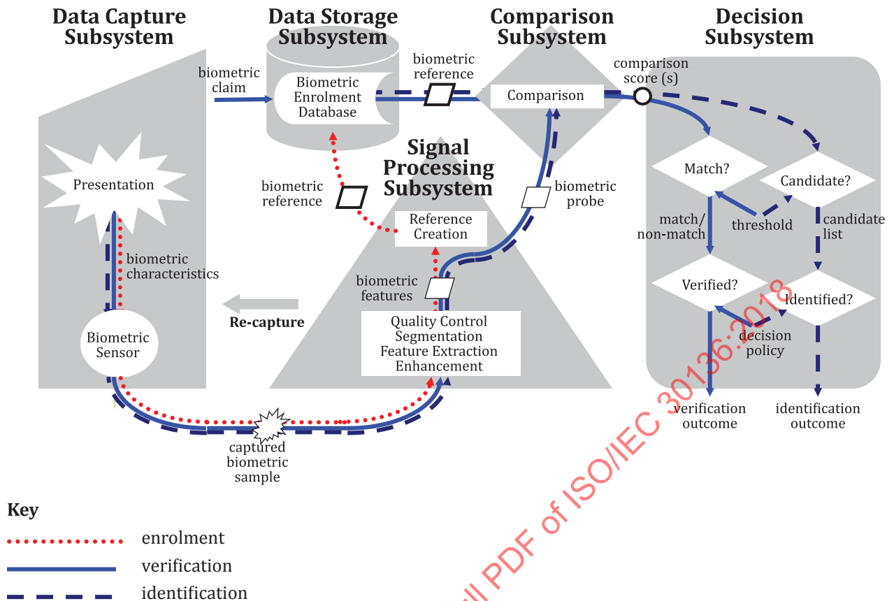
Figure 1 — Components of a conventional biometric system
