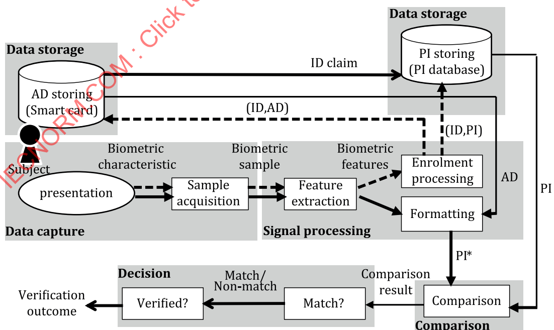
Figure 5 — Application model of two-factor biometric template protection system based on smart card
