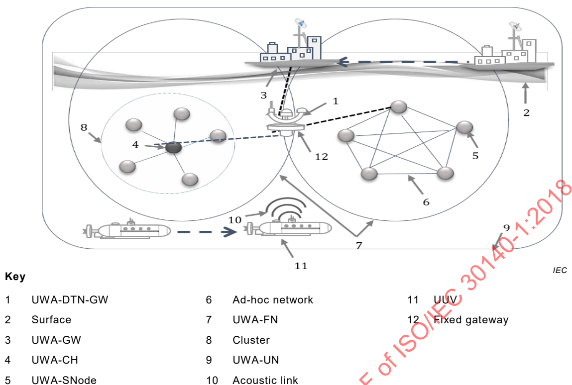
Figure 6 – UWA-UN communication network using fixed gateway
