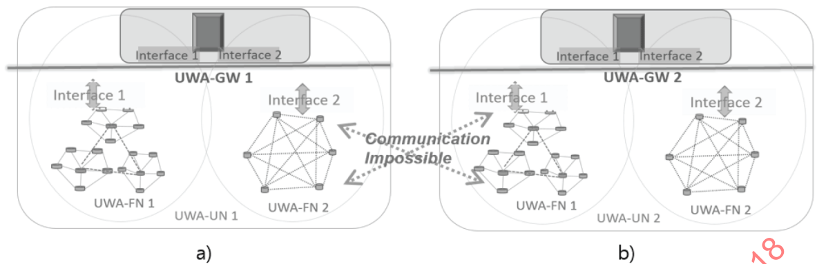
Figure 6 – Interoperability between fundamental networks
