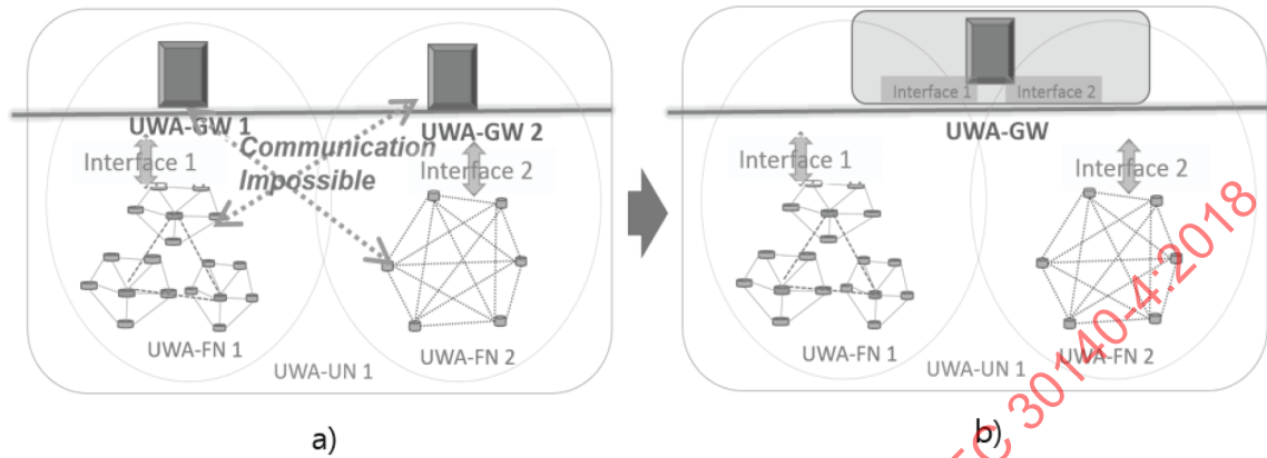
Figure 5 – Multiple interfaces on a UWA-GW to provide interoperability in UWASN
