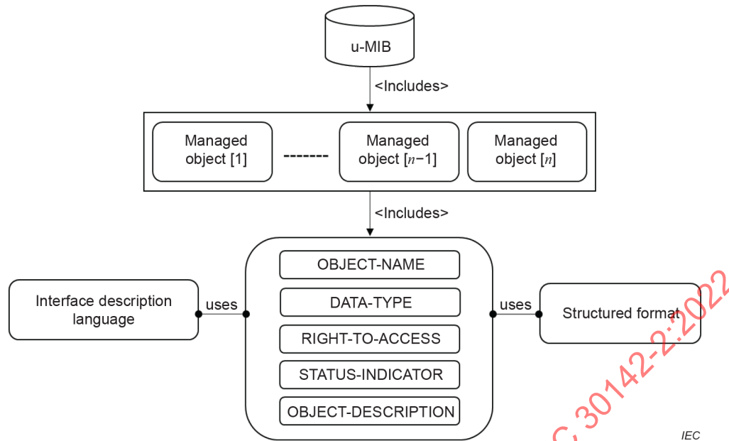
Figure 4 – General format of u-MIB
