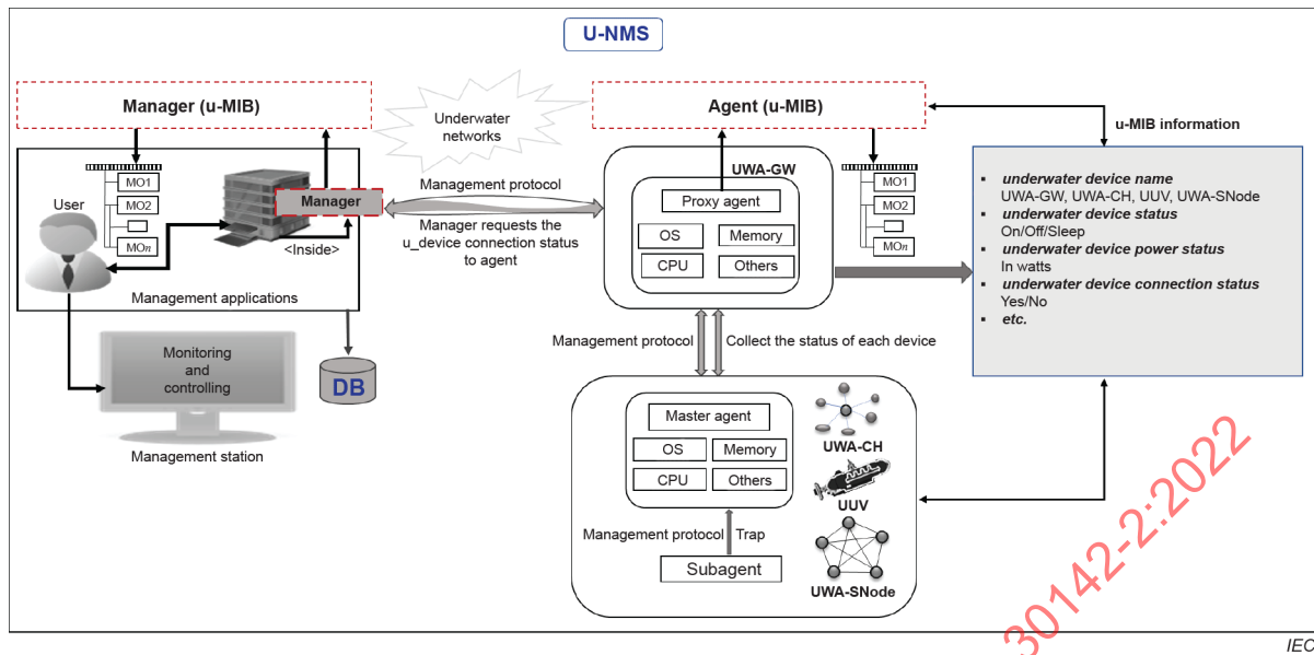
Figure 8 – MOs' requests via the network management protocol
