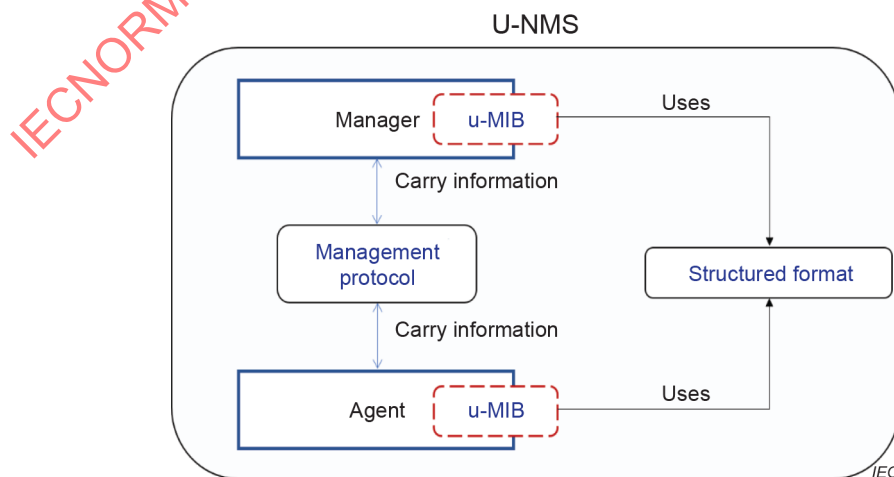
Figure 1 – Elements of u-MIB in U-NMS
