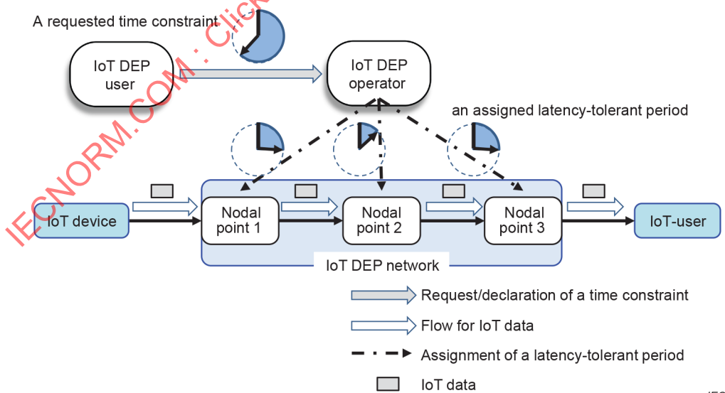
Figure B.1 – Assignment process of latency-tolerant periods
