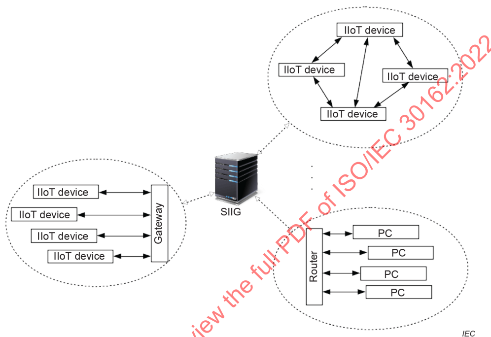
Figure 1 – A sample software/hardware set performing conversion between IIoT protocols using semantic Industrial Internet of Things gateway (SIIG)
