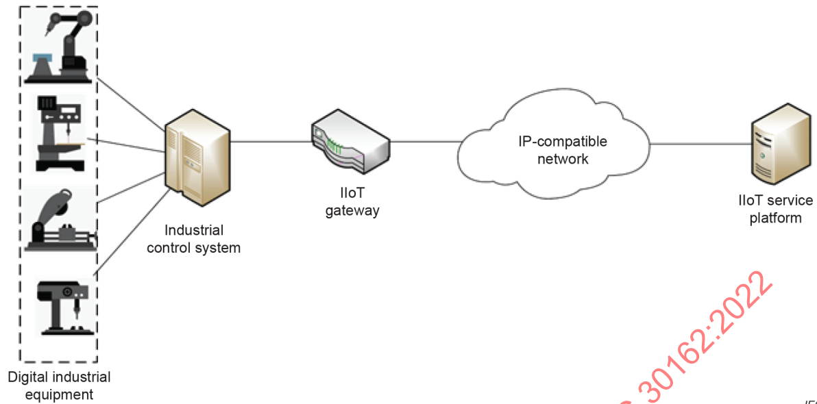
Figure 7 – Connectivity with an industrial control system
