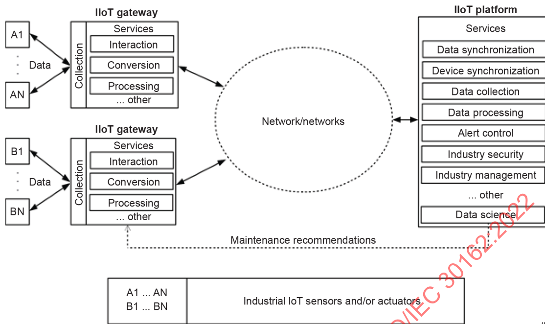
Figure 3 – IIoT system model with heterogeneous gateways
