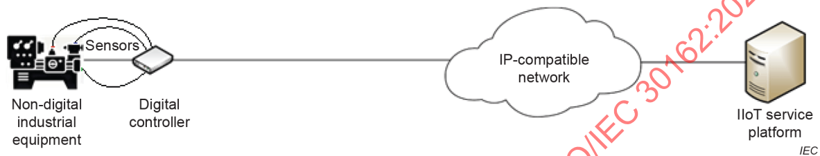
Figure 5 – Direct connectivity
