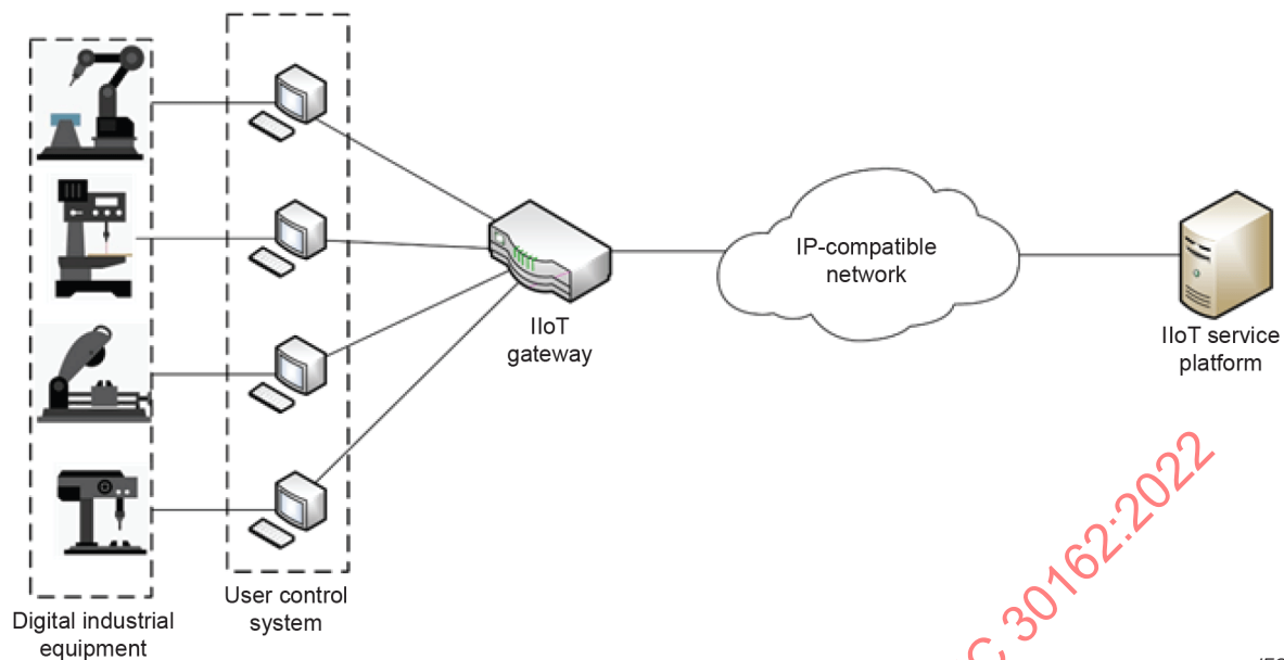
Figure 6 – Connectivity with IIoT gateway.
