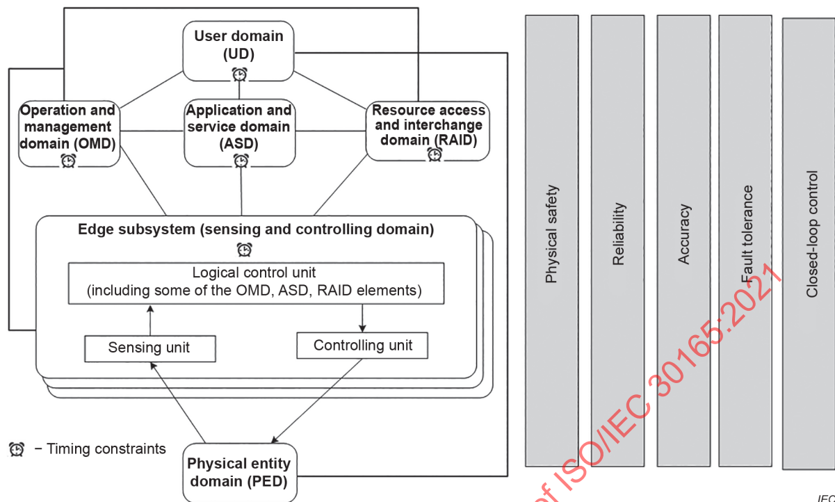
Figure 4 – RT-IoT system control view
