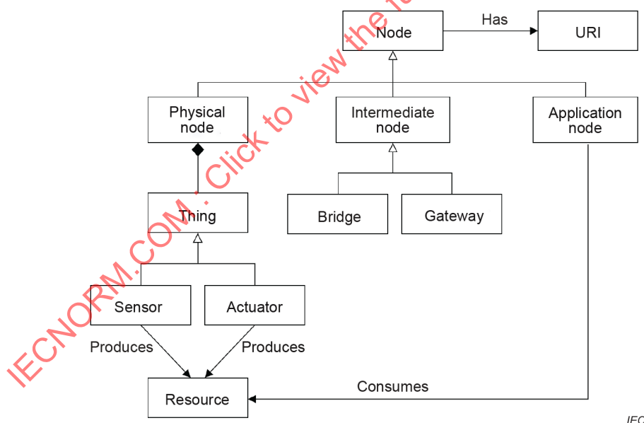
Figure 1 – The IoT metamodel
