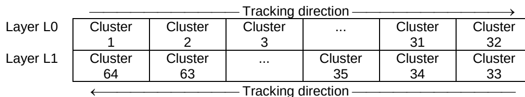
Figure 122 — Clusters of DMAs on DL disk
