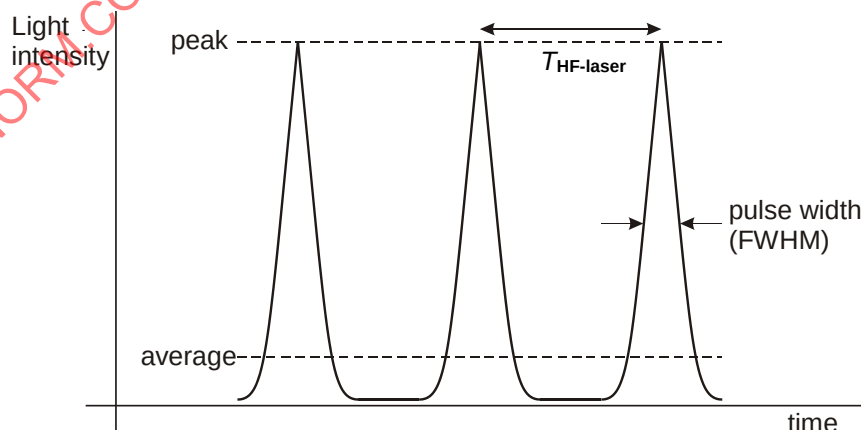
Figure 149 — Schematic representation of light pulses from Laser Diode
