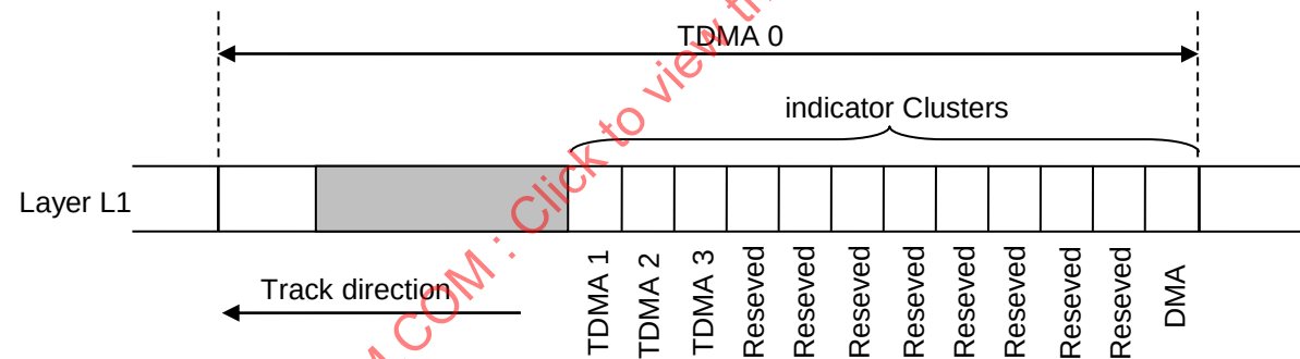
Figure 119 — TDMA Indicator Clusters on QL disk
