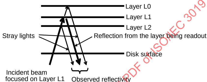
Figure B.2 — Influence of stray lights from other layers
