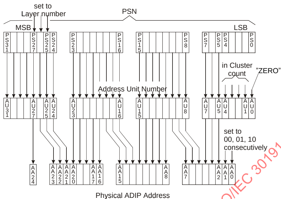
Figure 92 — Physical ADIP Addresses derived from PSN's
