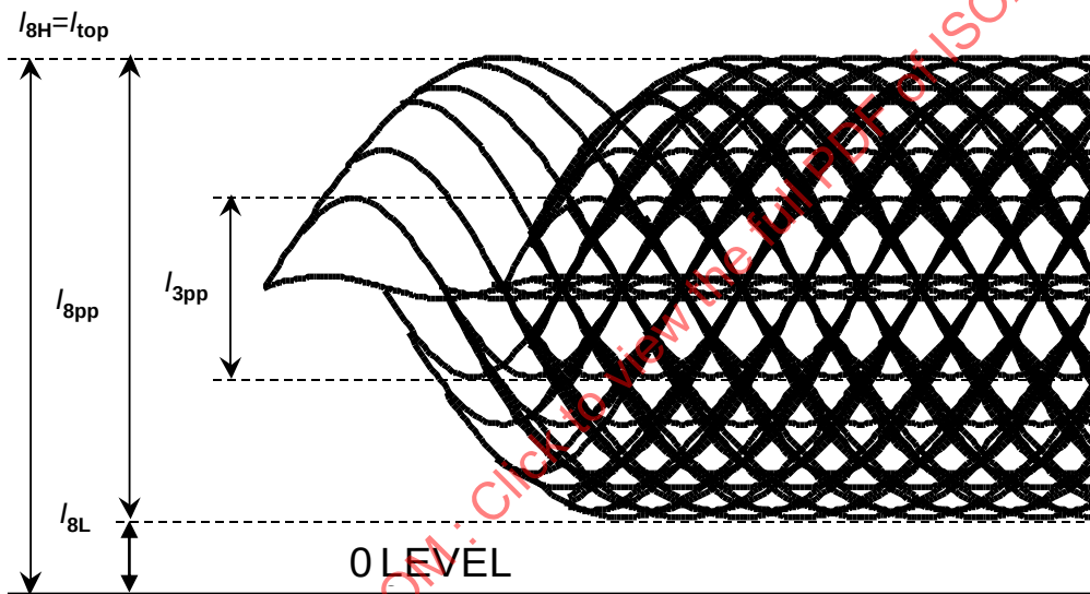
Figure 147 — Schematic representation of HF signal from Marks and Spaces
