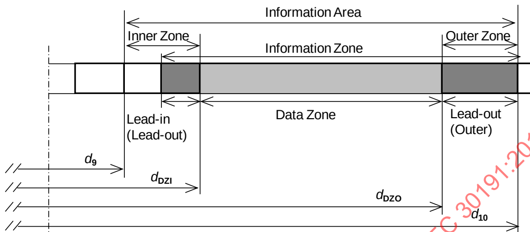
Figure 14 — Division of Information Area
