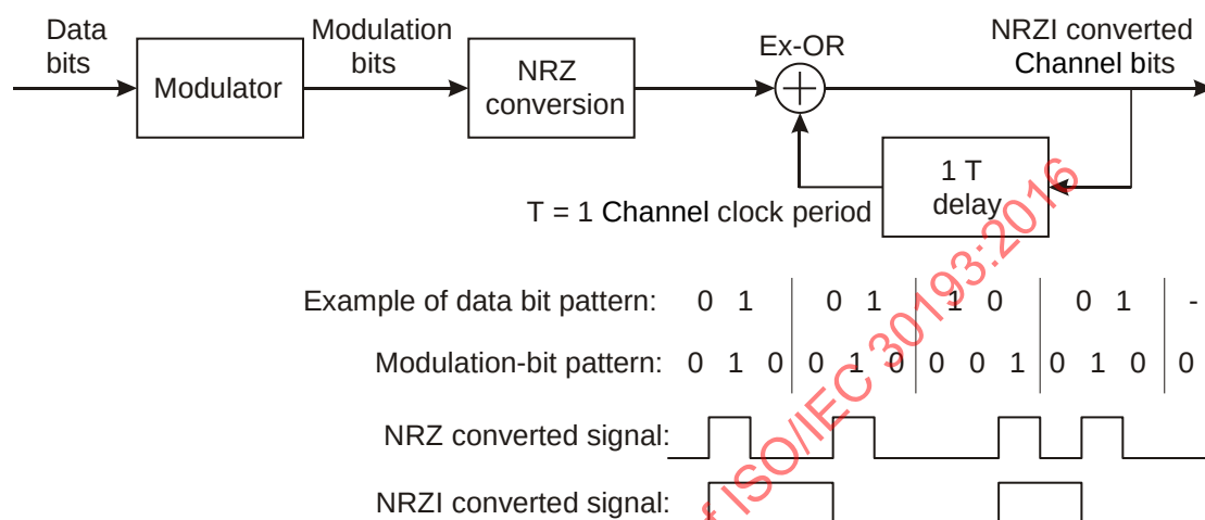
Figure 40 — Modulation and NRZI conversion
