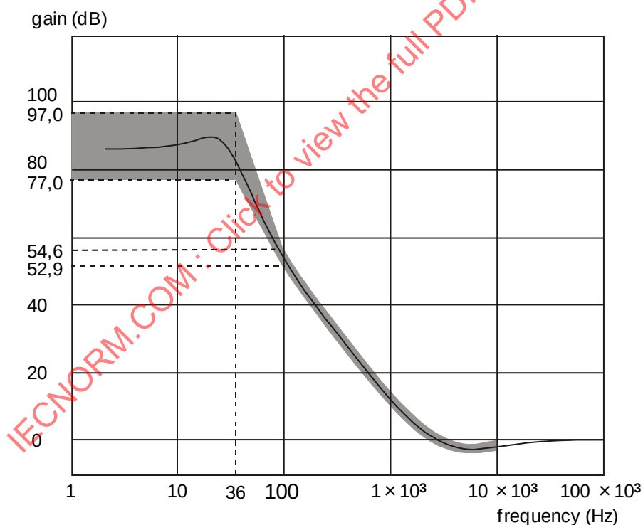
Figure 6 — Servo characteristic for axial tracking
