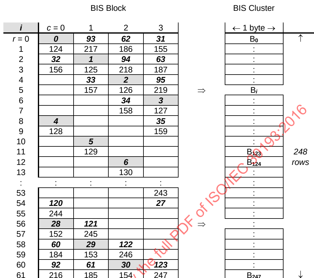
Figure 57 — Reading order for constructing PIC BIS Cluster
