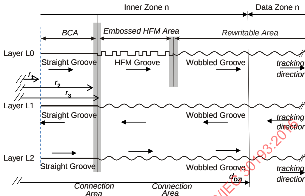
Figure 52 — Connection Areas between different Groove Types
