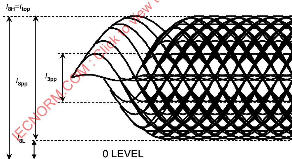
Figure 119 — Schematic representation of HF signal from Marks and Spaces
