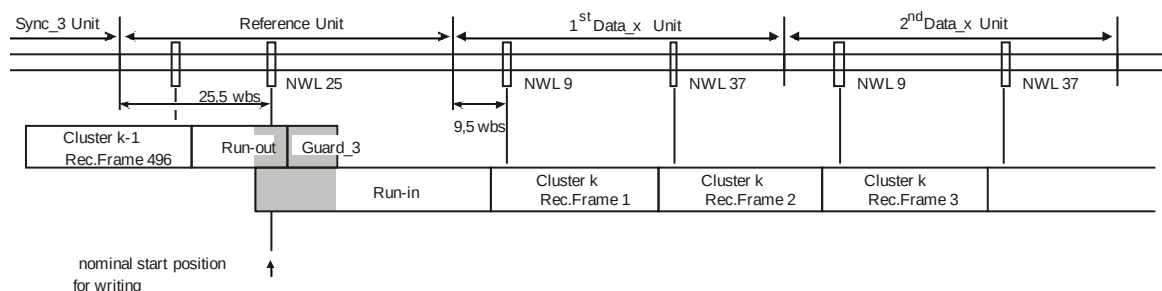
Figure 50 — Example of data recording with maximum overlap
