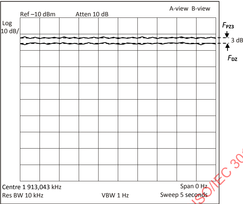
Figure E.3 — Example of fundamental wobble frequency level measurement
