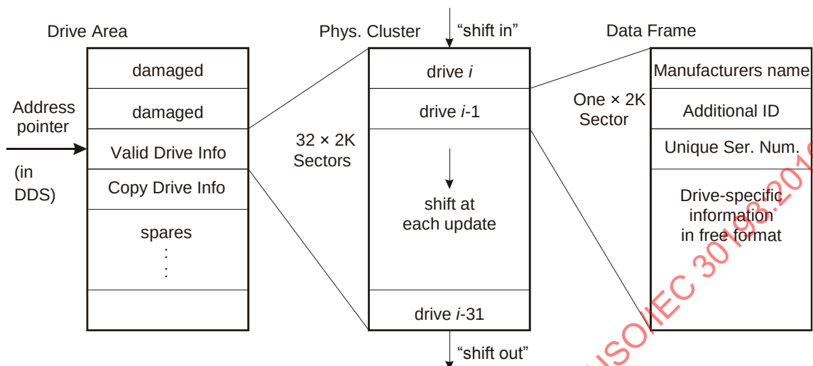
Figure 91 — Format of Drive Area (example)
