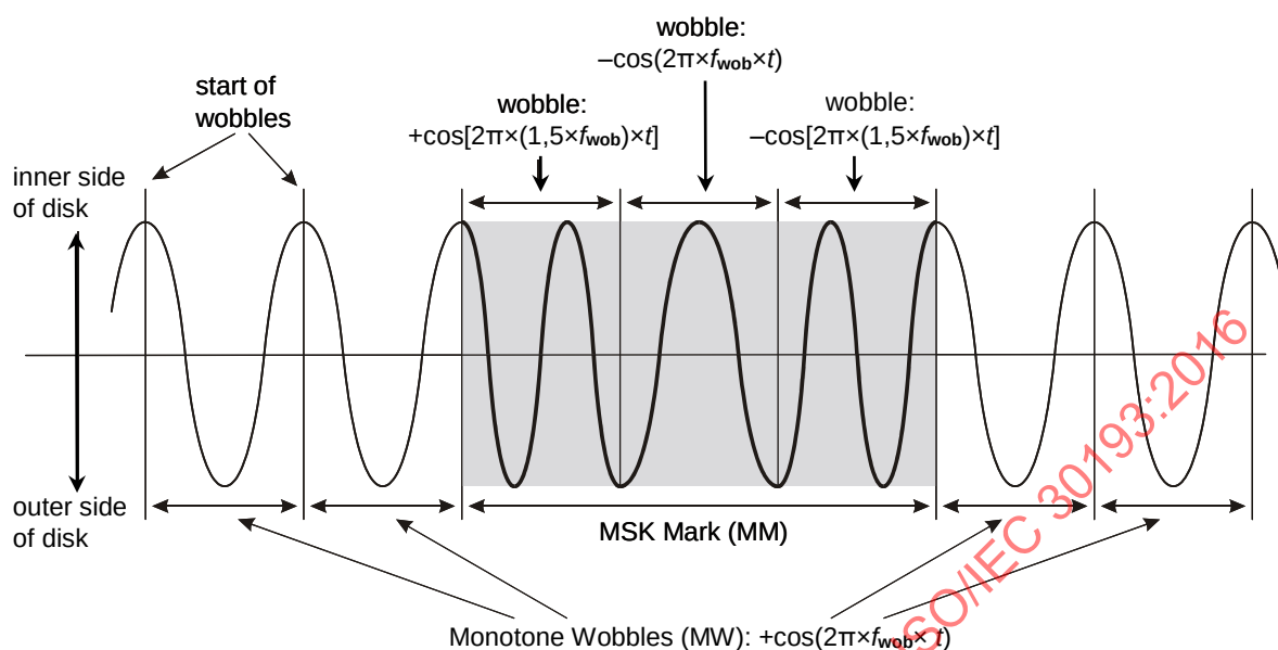
Figure 62 — Definition of MSK Mark (on Groove)
