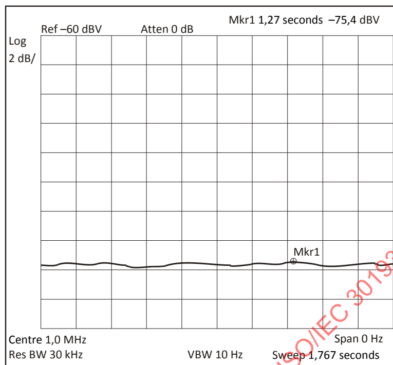
Figure E.2 — Example of spectrum analyzer showing noise signal
