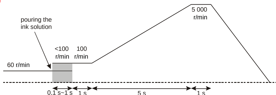
Figure D.4 — Speed profile for spin coating ink pad
