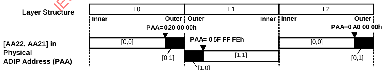
Figure 68 — Relation between PAA and PAS
