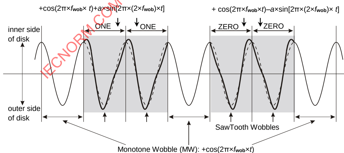
Figure 63 — Definition of Saw-Tooth Wobblers (on-Groove)
