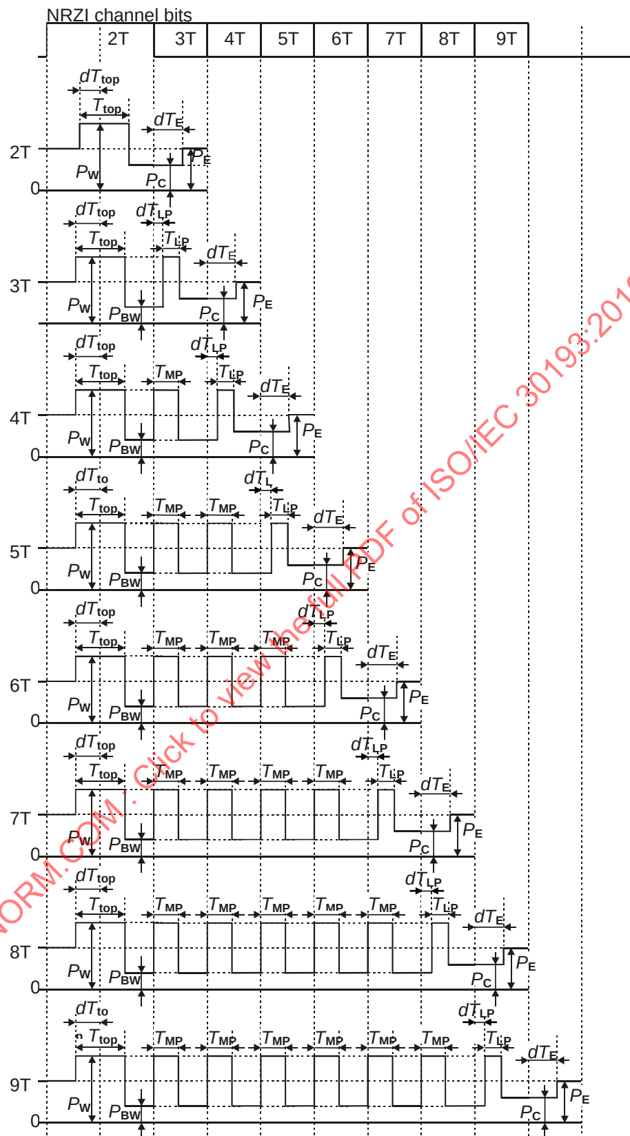
Figure F.1 — General write-pulse waveform for Extended N-1 write strategy
