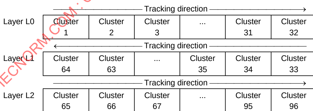
Figure 103 — Clusters of DMA Zones
