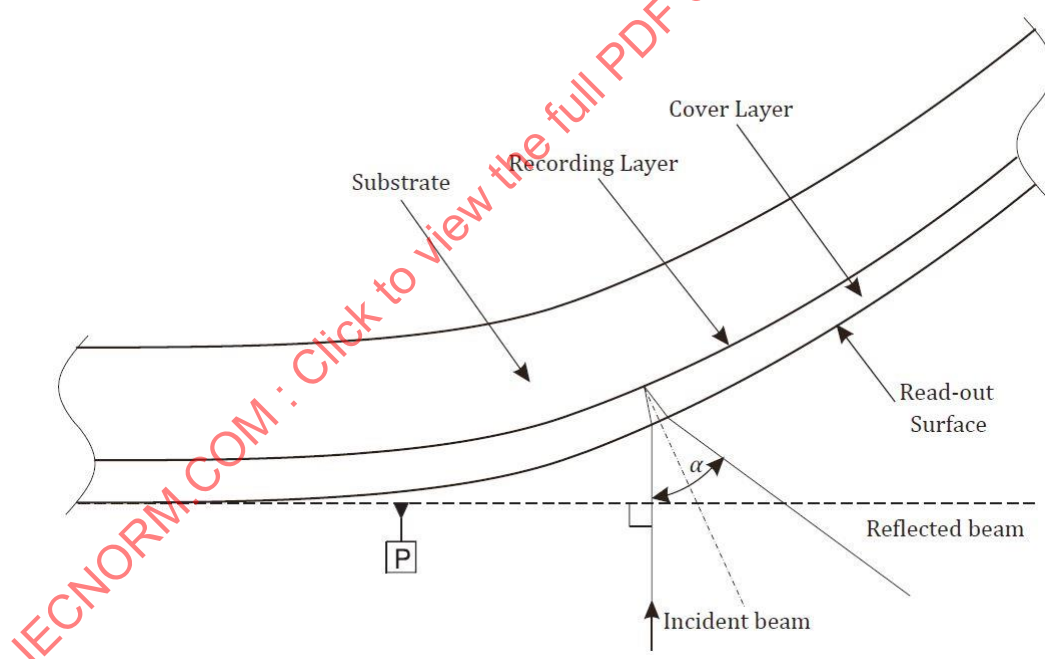
Figure 15 — Definition of angular deviation
