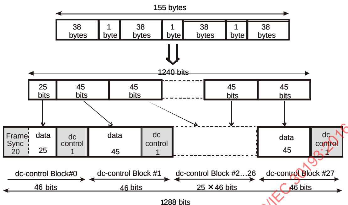
Figure 35 —Composition of Recording Frame
