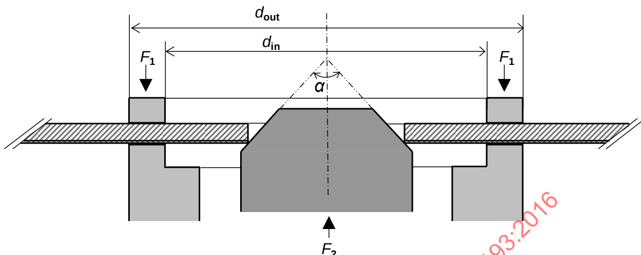
Figure 5 — Clamping conditions for measurement
