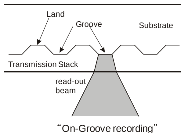
Figure 53 — Outline of Groove geometry (Radial cross-section of disk)
