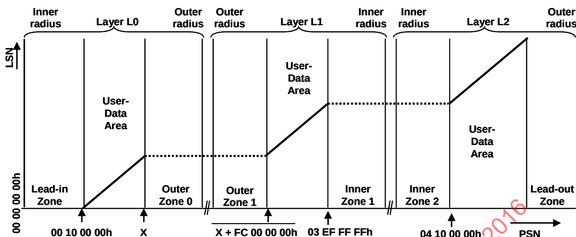
Figure 116 — Assignment of Logical-Sector Numbers
