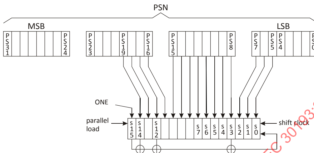
Figure 19 — Scrambler circuit
