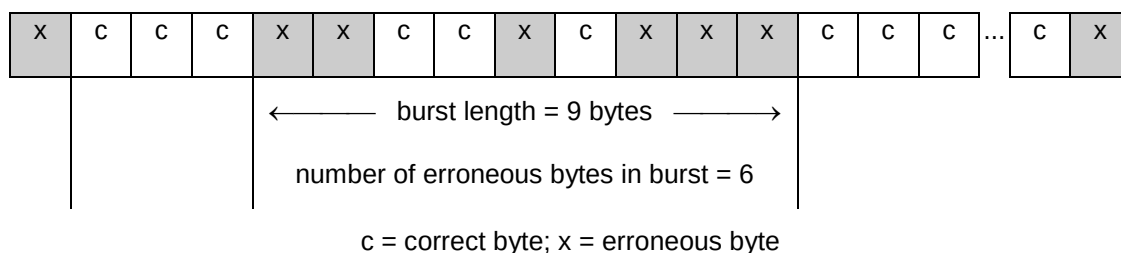
Figure 121 — Example of burst error
