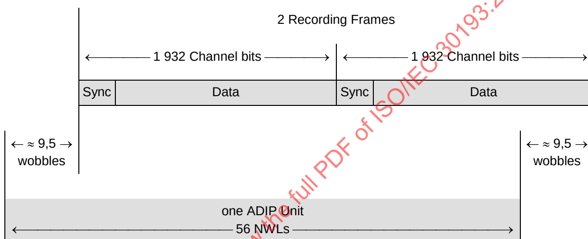
Figure 64 — General ADIP structure
