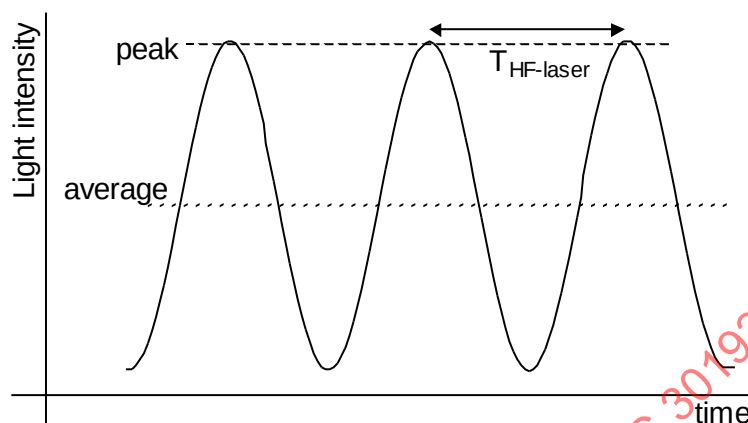
Figure 120 — Schematic representation of light pulses from Laser Diode
