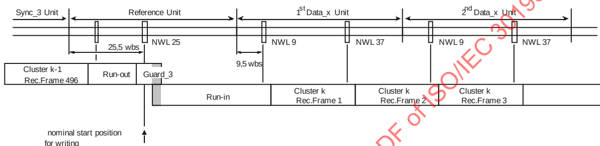
Figure 51 — Example of data recording with minimum overlap
