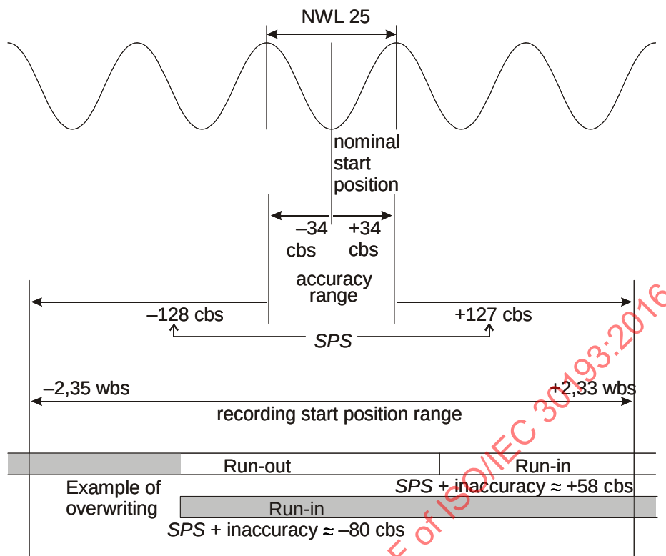
Figure 48 — Nominal start position for data recording
