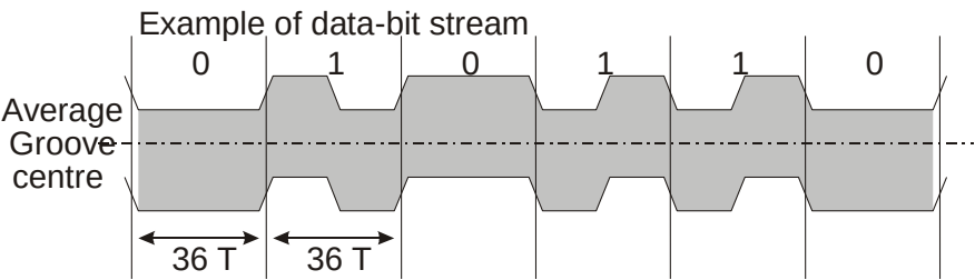
Figure 58 — Biphase modulated HFM Groove
